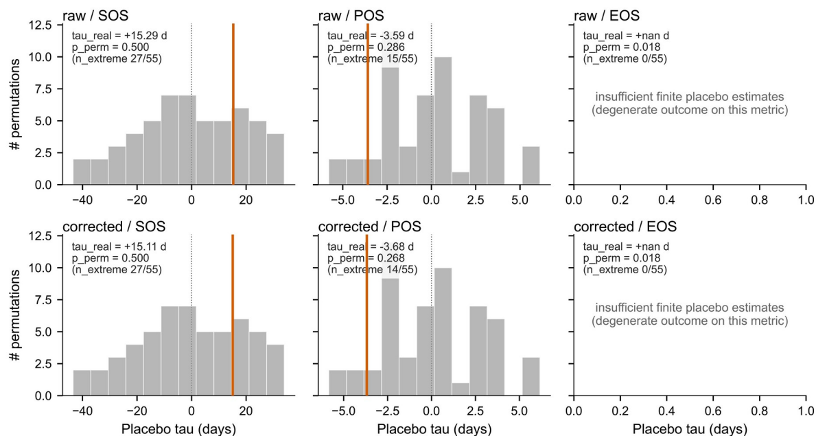
Figure 6. Placebo distribution under random treatment assignment.
