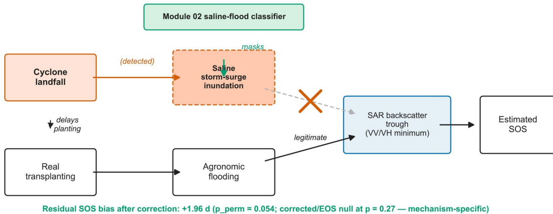
Figure 1B. Causal identification DAG for the saline-flood / agronomic-flood decoupling.
