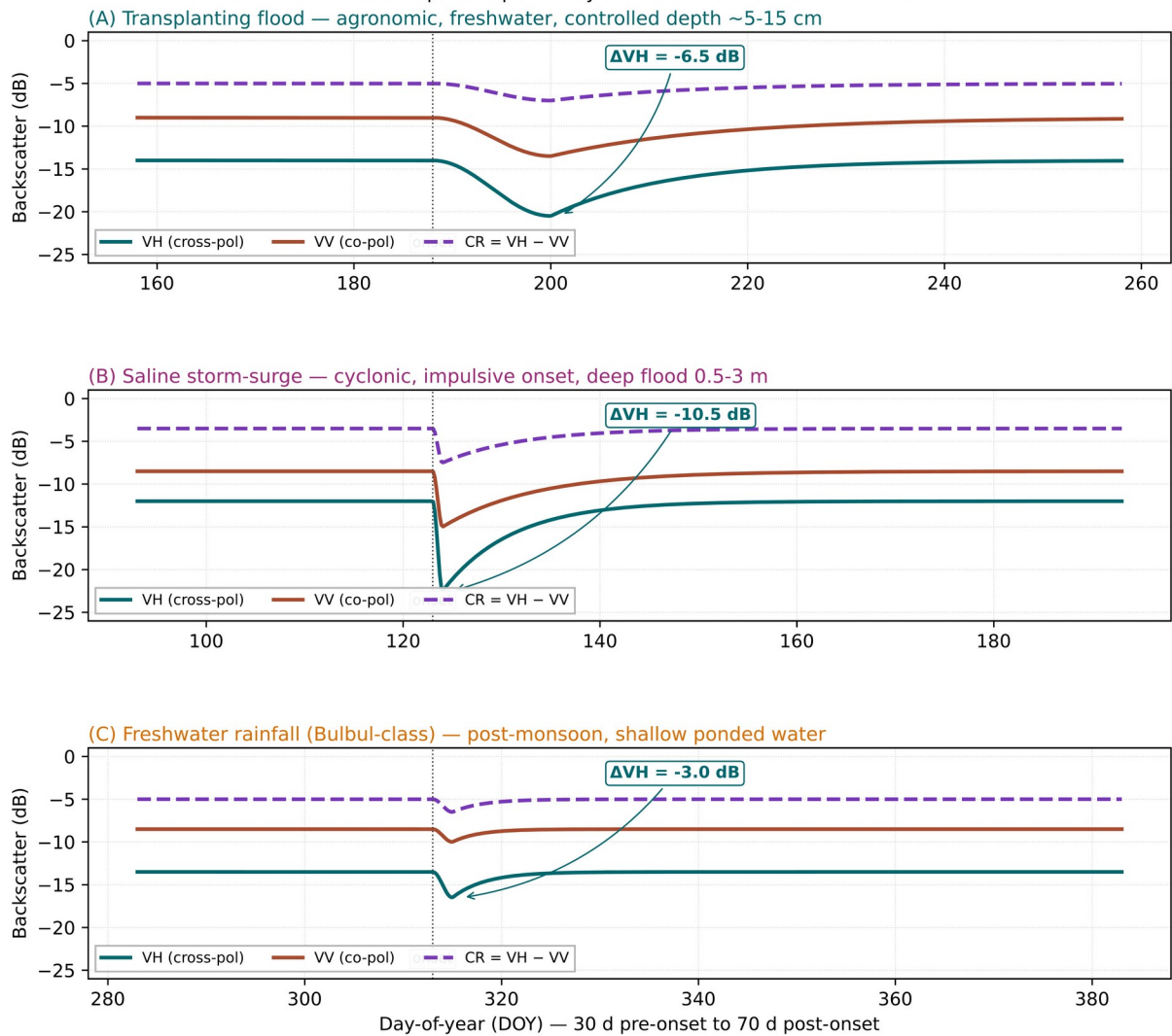
Figure S2. Canonical Sentinel-1 dual-polarisation backscatter signatures for the three inundation mechanisms. Differentiable feature space exploited by the Module 02 random-forest classifier.
