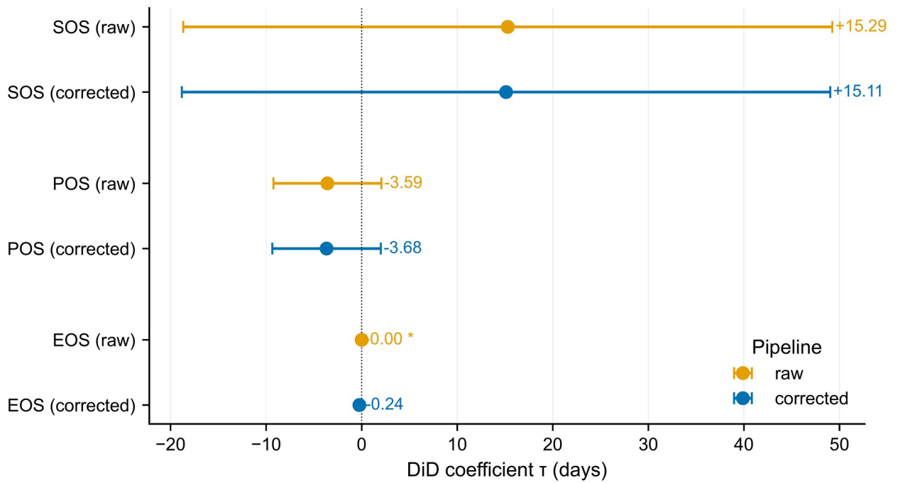
Figure 2. TWFE-DiD coefficients (raw vs. classifier-corrected panel).
