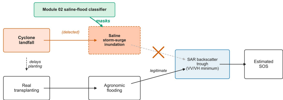
Figure 1B. Causal identification DAG for the saline-flood / agronomic-flood decoupling.
