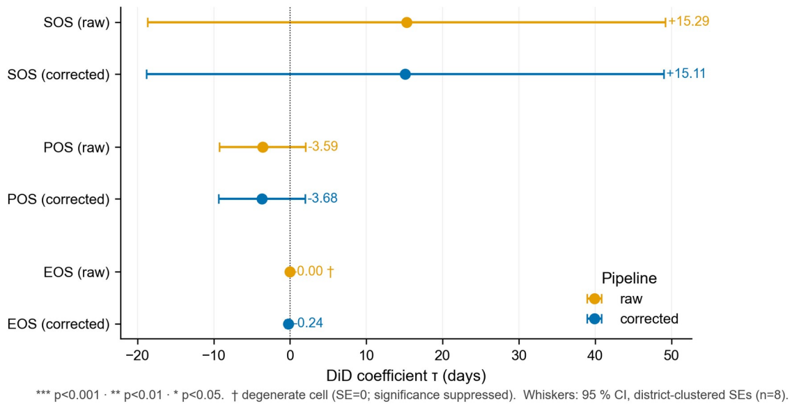
Figure 3. TWFE-DiD coefficients (raw vs. classifier-corrected panel). Point estimates with district-clustered (CR1) standard-error bars and 95% wild-cluster restricted bootstrap intervals for SOS, POS, and EOS, raw and corrected pipelines on the real v2.1 panel.
