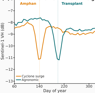
(A) Two flood events • one SAR signal
