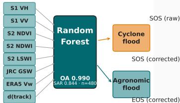
(B) 8-feature RF classifier
