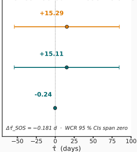
(C) BACI-corrected DiD coefficients
