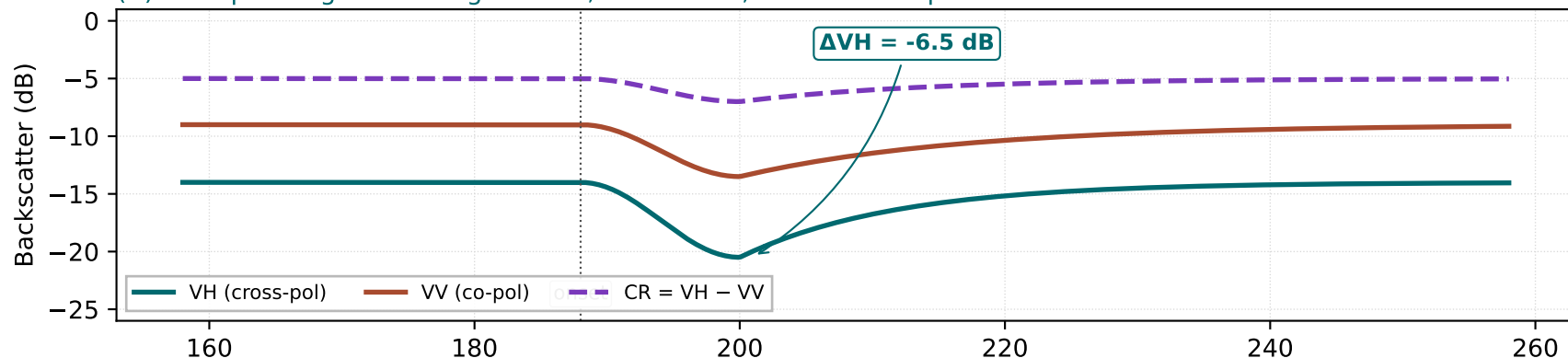
Figure S2. Canonical Sentinel-1 dual-polarisation backscatter signatures for the three inundation mechanisms. Differentiable feature space exploited by the Module 02 random-forest classifier.
