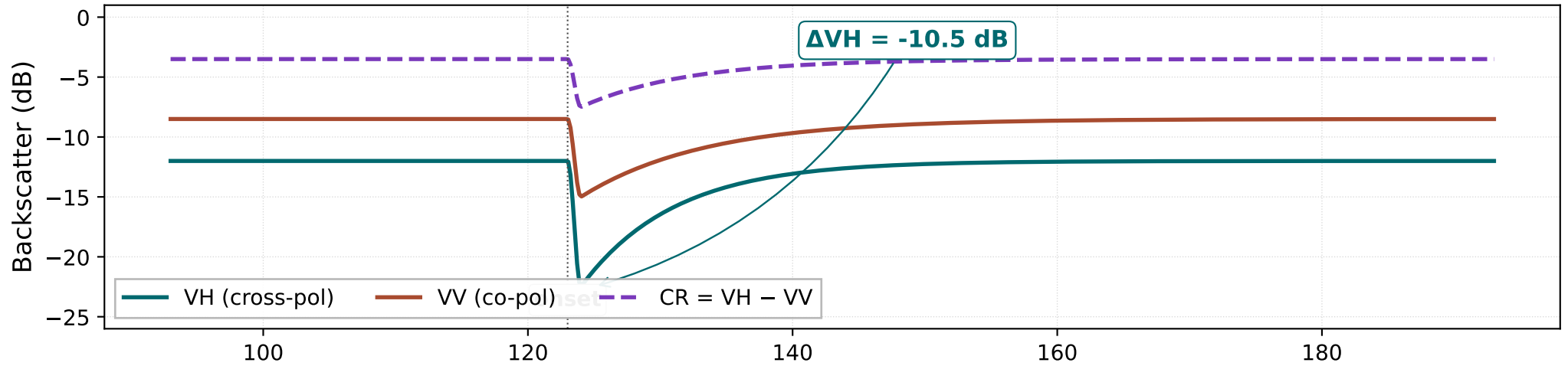
(B) Saline storm-surge — cyclonic, impulsive onset, deep flood 0.5-3 m
