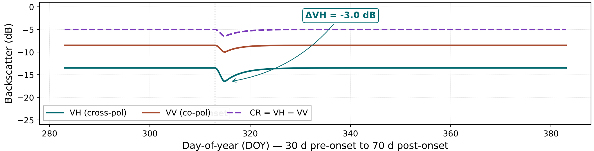
(C) Freshwater rainfall (Bulbul-class) — post-monsoon, shallow ponded water
