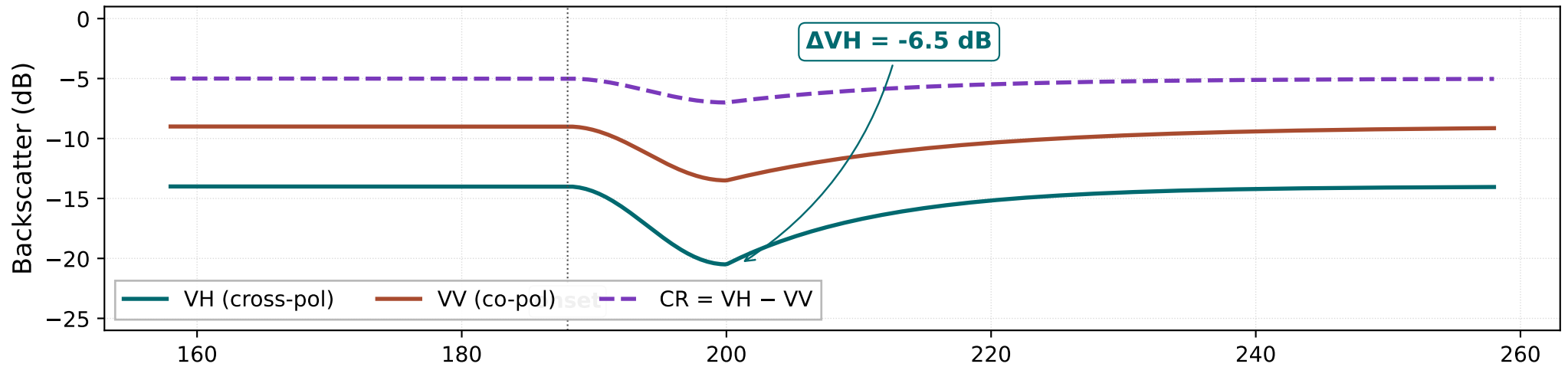
(A) Transplanting flood — agronomic, freshwater, controlled depth ~5-15 cm
