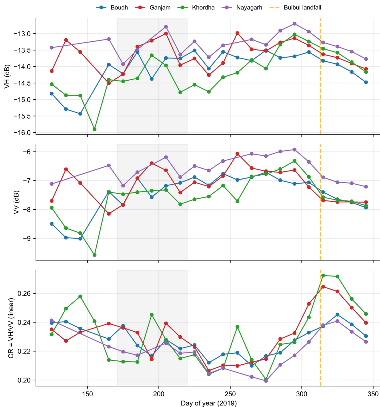
Figure S2. Real Sentinel-1 RTC dual-pol backscatter time series across the four Bulbul probe districts (Boudh, Ganjam, Khordha, Nayagarh) for the 2019 Kharif/post-monsoon window, retrieved from the Microsoft Planetary Computer sentinel-1-rtc collection ( n = 85 district-dekads, 334 scenes). Top: VH (cross-pol, dB). Middle: VV (co-pol, dB). Bottom: CR = VH/VV (linear). Shaded band indicates the agronomic transplanting window (DOY 171–220); dashed vertical line marks Cyclone Bulbul landfall (9 November 2019, DOY 313).
