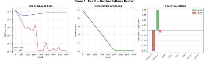
Fig. 7. Variant R3 with stochastic Gumbel-Softmax sampling at validation time. The validation curve shows order-of-magnitude excursions at individual logging epochs (e.g., epoch 1,600 reading 1.9 \times 10^{-3} between 10^{-6} neighbours) caused by single unlucky Gumbel draws.
