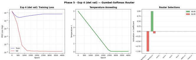
Fig. 9. Variant R3 under deterministic validation evaluation. The training curve climbs as the entropy and complexity penalties scale up with the temperature schedule; the validation curve, free of Gumbel noise, decays monotonically to the floor of 10^{-6} .
