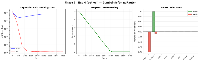
Fig. 10. Variant R4 under deterministic validation evaluation. The routing architecture is identical to R3; differences lie entirely in the entropy formulation and the complexity prior strength.
