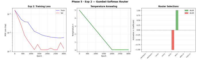
Fig. 6. Variant R2 (state-independent router): the router converges to \sin rather than identity, illustrating the \sin(z) \approx z collinearity at small |z| that motivates the complexity prior in R3. Validation MSE plateaus at \approx 1.2 \times 10^{-3} , dominated by the missing damping term.
