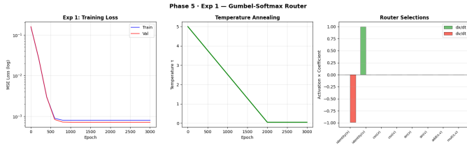
Fig. 5. Variant R1 (state-dependent router): training/validation curves and routing summary. The router commits to \text{identity}(v) for \dot{x} and \text{identity}(x) for \dot{v} , but k=1 selection precludes recovery of the damping component, leaving val MSE at \approx 7.2 \times 10^{-4} .
