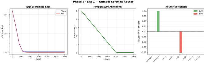
Fig. 5. Variant R1 (state-dependent router): training/validation curves and routing summary. The router commits to identity( v ) for \dot{x} and \sin(x) for \dot{v} ; k=1 selection precludes recovery of the damping component, leaving val MSE at \approx 9.8 \times 10^{-4} .
