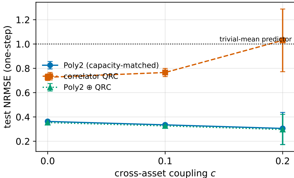
Case I: correlator QRC vs. polynomial control
