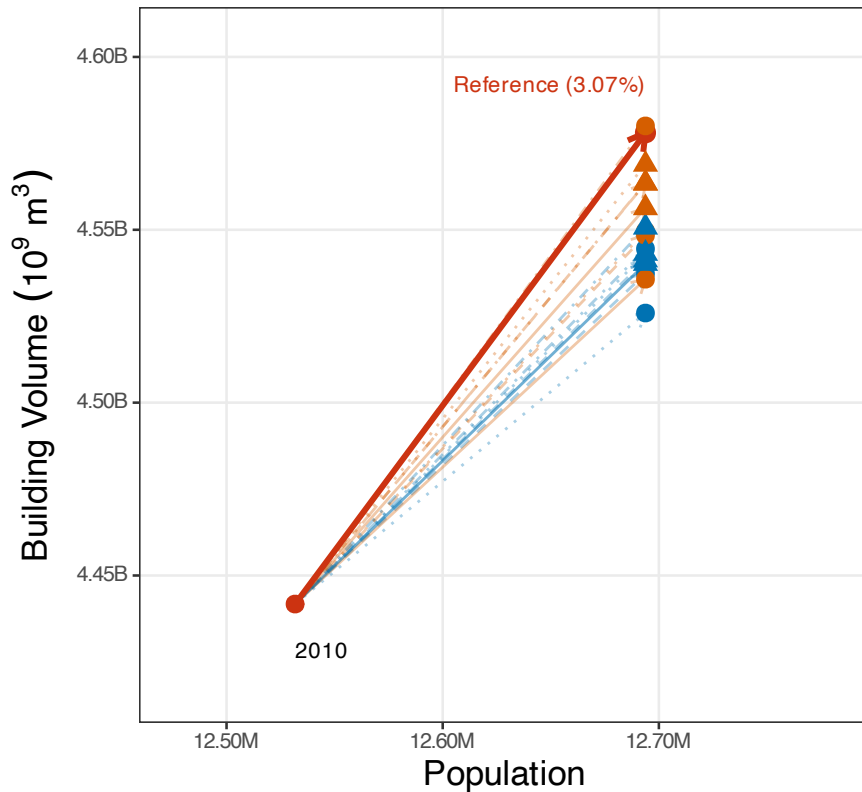
Los Angeles Urban Area 2010-2020 Growth
