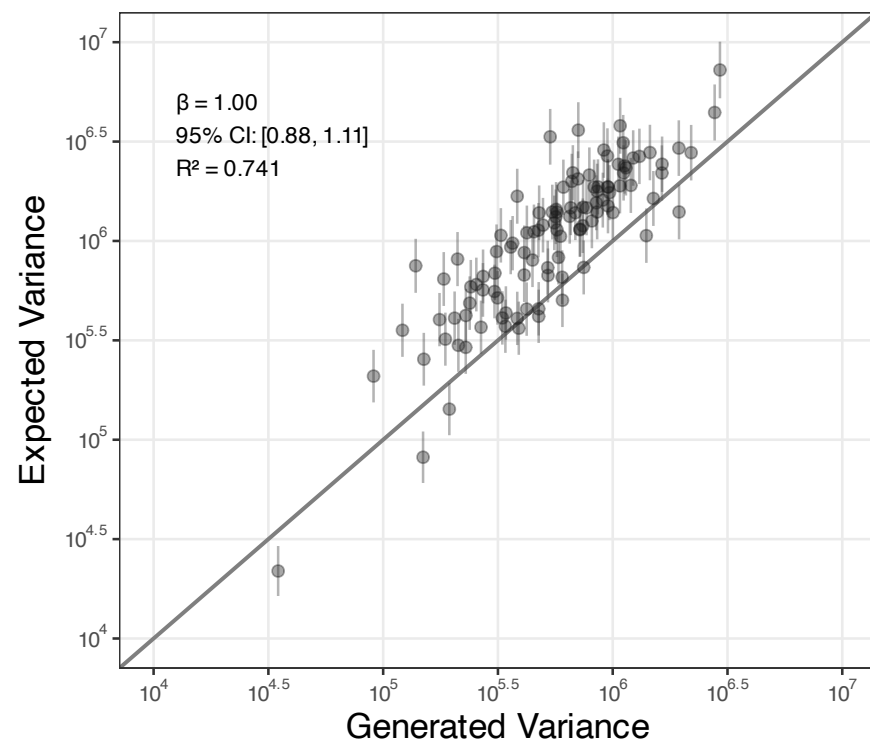
Single-Latent LA Model (LR = 0.0002)
