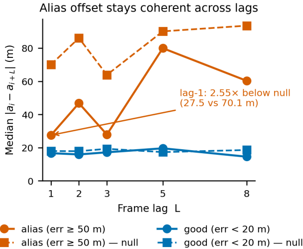
Fig. 6. Temporal coherence of the alias offset (R04, n = 610 contiguous). Solid: median pairwise offset difference within the alias ( \geq 50 m) and good ( < 20 m) groups; dashed: shuffled nulls. The alias group sits 2.55\times below its null at lag 1 and decays to \sim 1.1\times by lag 5–8; correct fixes are independent at every lag.
