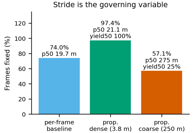
Fig. 8. Stride governs availability: per-frame baseline, dense propagation (3.8 m), and coarse propagation (250 m) on 429 video-rate frames.
