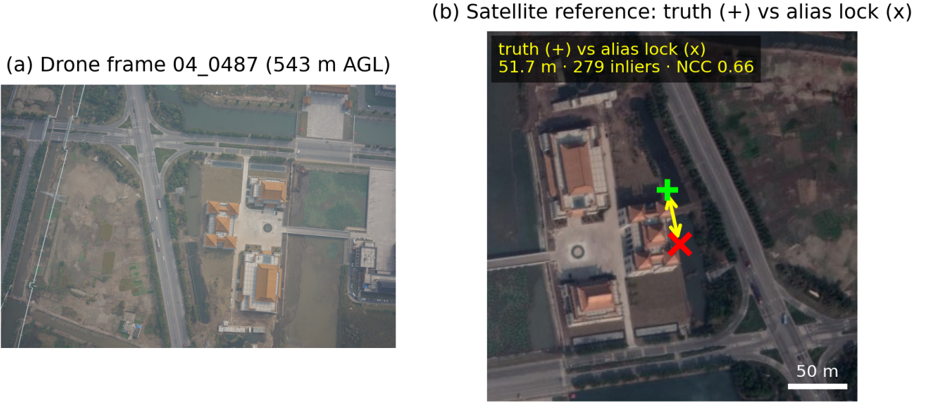
Fig. 4. The smoking-gun frame (R04, 04_0487). (a) Drone view at 543 m AGL. (b) Satellite reference crop: the accepted lock (279 inliers, NCC 0.66) sits 51.7 m from GPS truth along the field structure.
