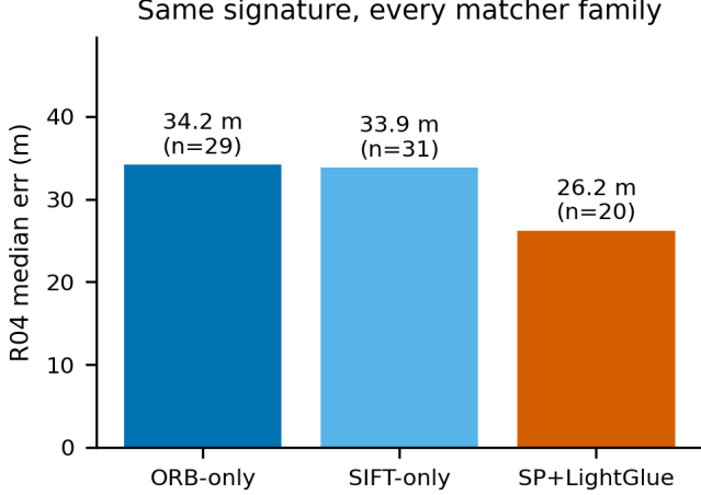
Fig. 7. R04 median error is matcher-independent across classical and learned families (LightGlue cells underpowered, reported as such).
