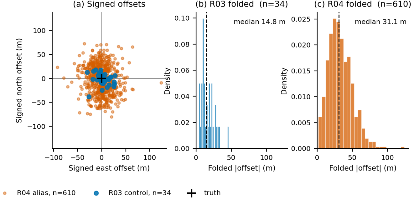
Fig. 3. The sign-folding diagnostic. Left: signed (north, east) offsets on R04 ( n = 610 contiguous) and R03 (step-sampled). The R04 alias class is axis-aligned with a hole at zero; R03 is unstructured. Right: the same R04 data folded to magnitudes—the standard reporting convention—appears continuous and hides the alias class.
