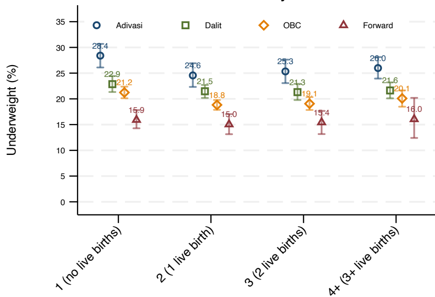
C. Parity
