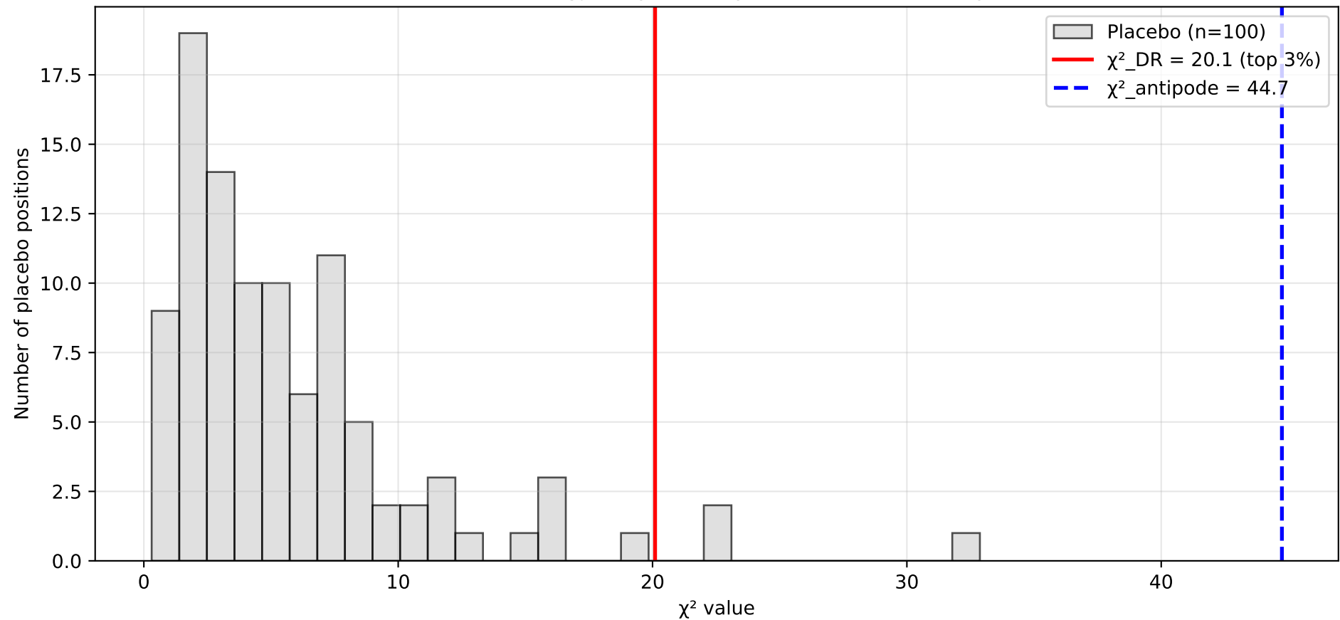
Distribution of \chi^2 for placebo positions vs DR / antipode
