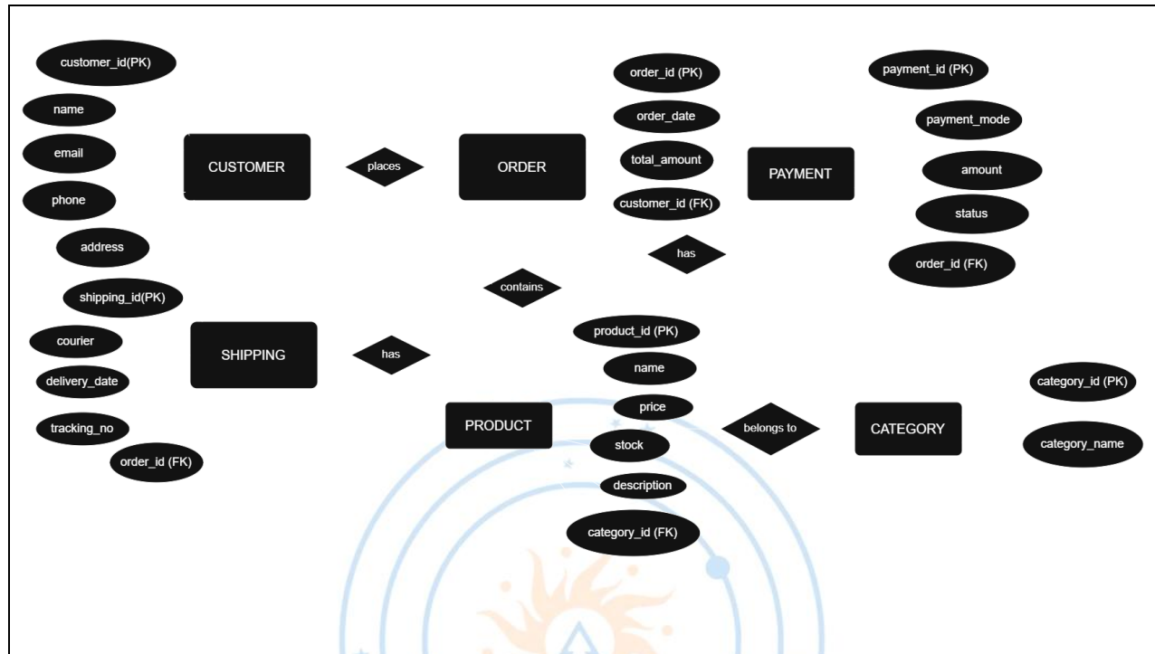
Fig. 3.1: ER Diagram of the Online Shopping System
