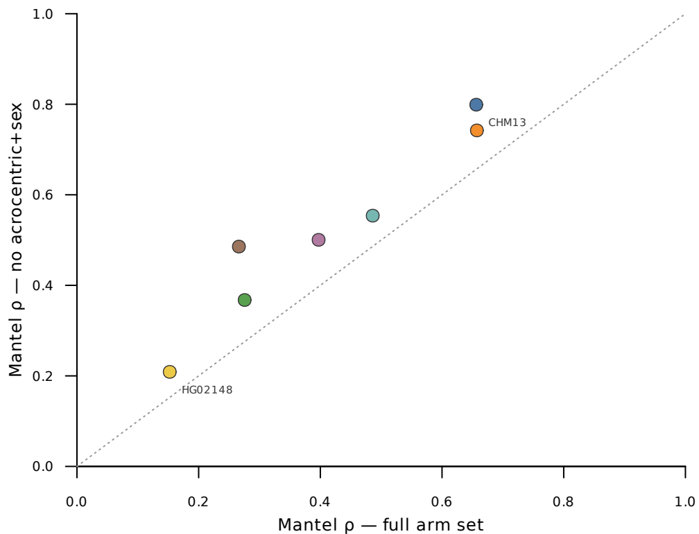
b Mantel \rho — full vs no acro/sex (50 kb)
