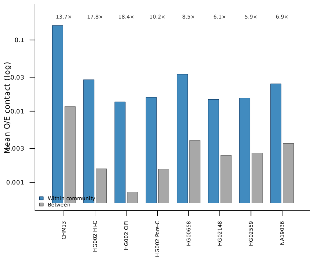
c O/E contact (mean): within vs between sequence community
