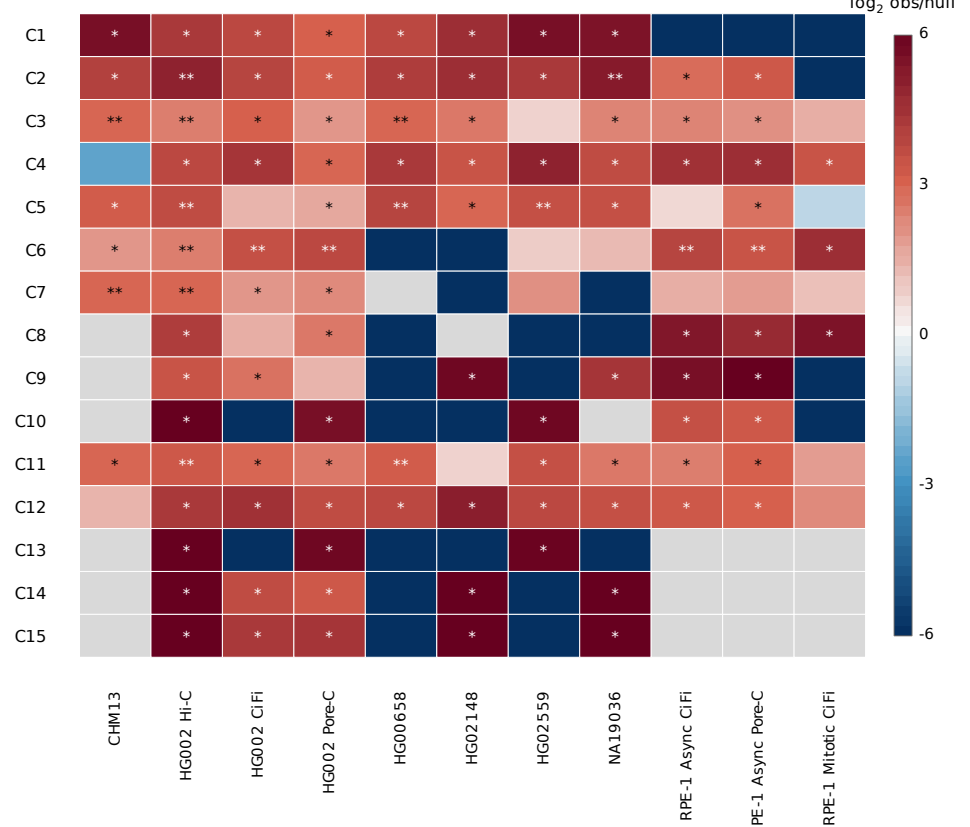
d Per-community enrichment (15 × 11; * q < 0.05 , ** q < 0.001 )
