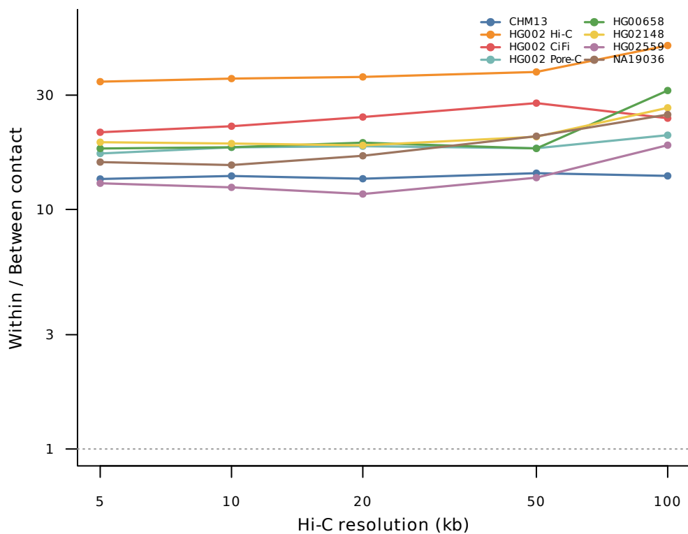
a Within/Between contact across 5 mcool resolutions
