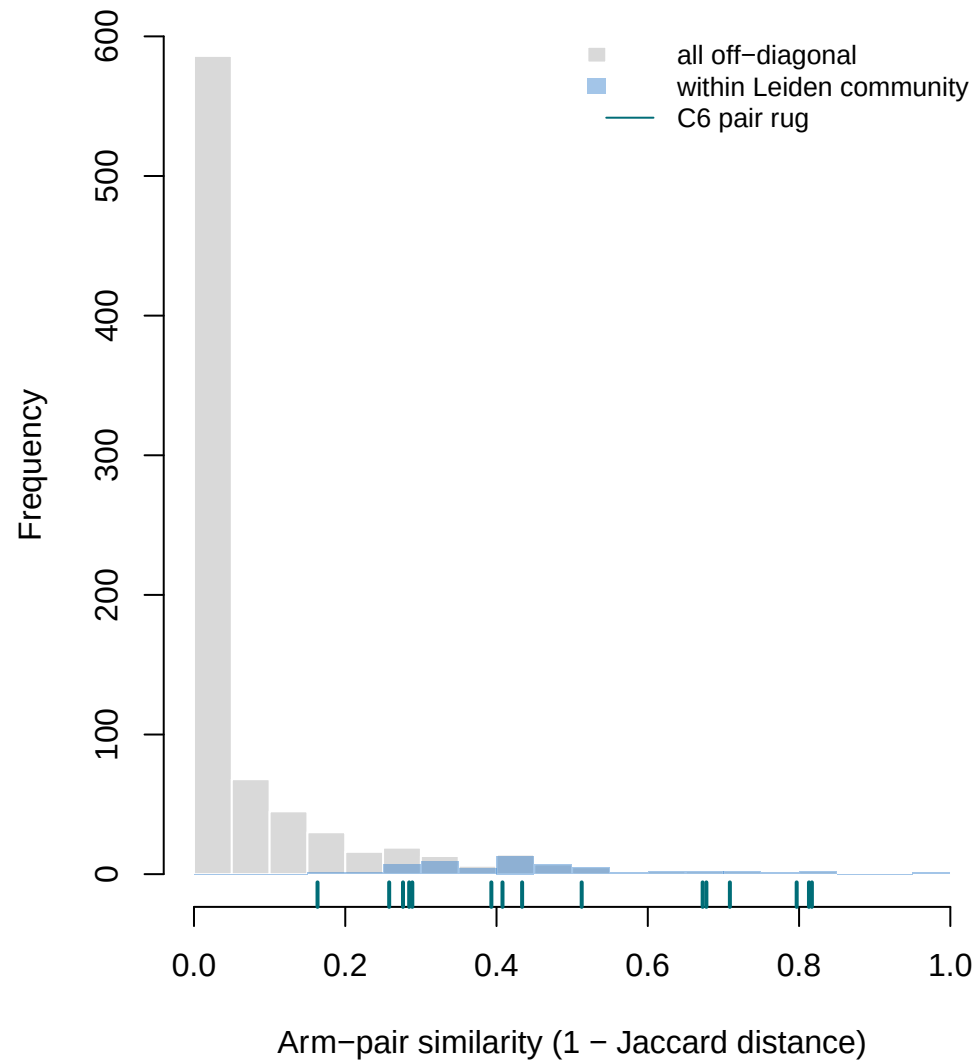
Off-diagonal distribution
