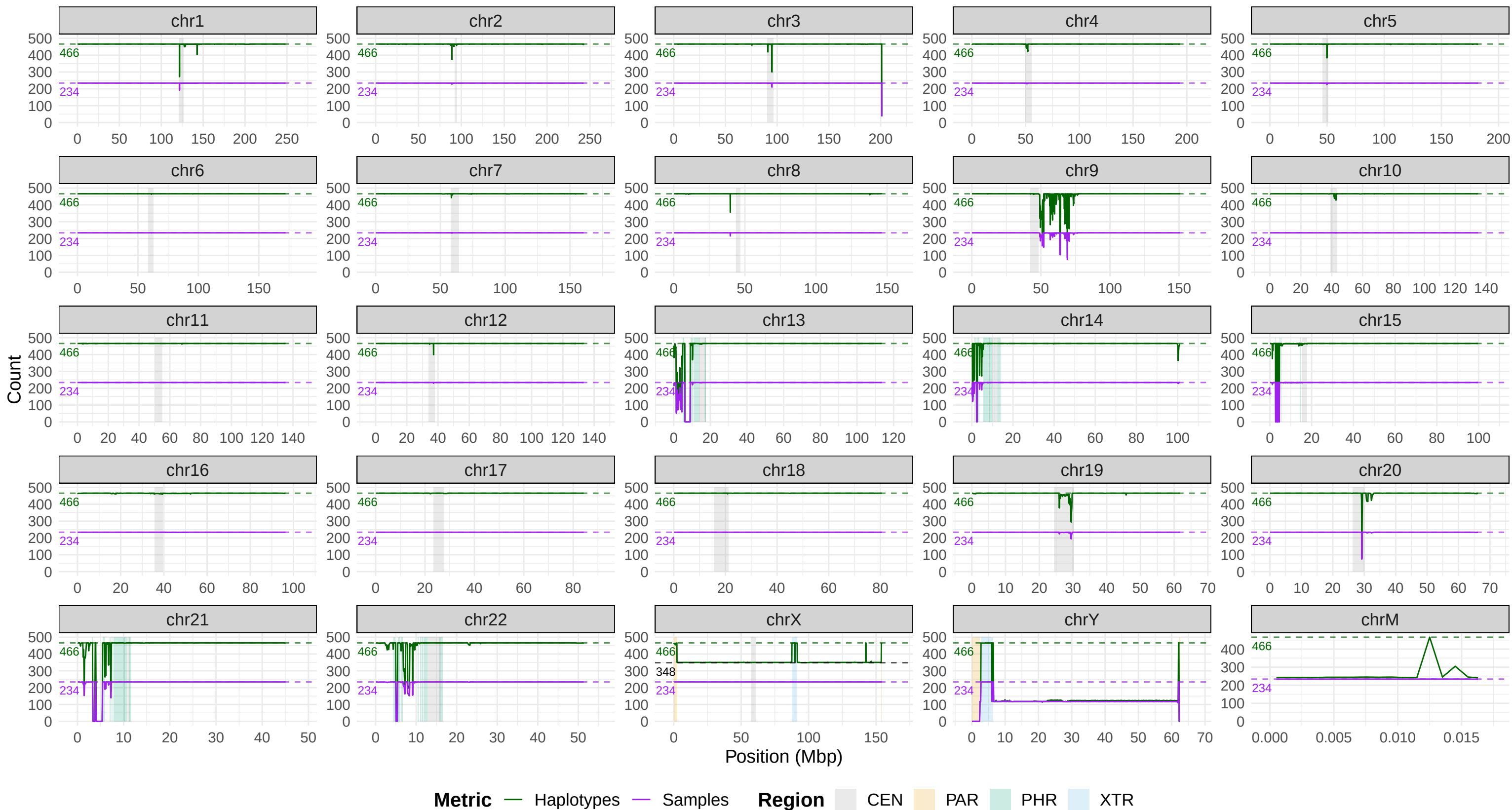
Samples/Haplotypes across CHM13 (100kb windows)
