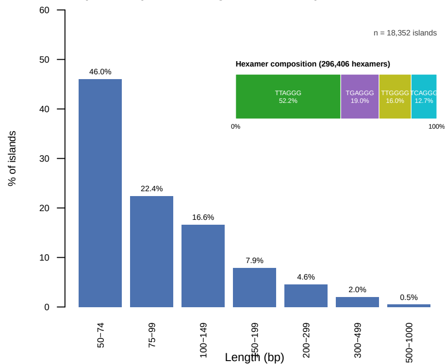
b (TTAGGG)n island length + motif composition
