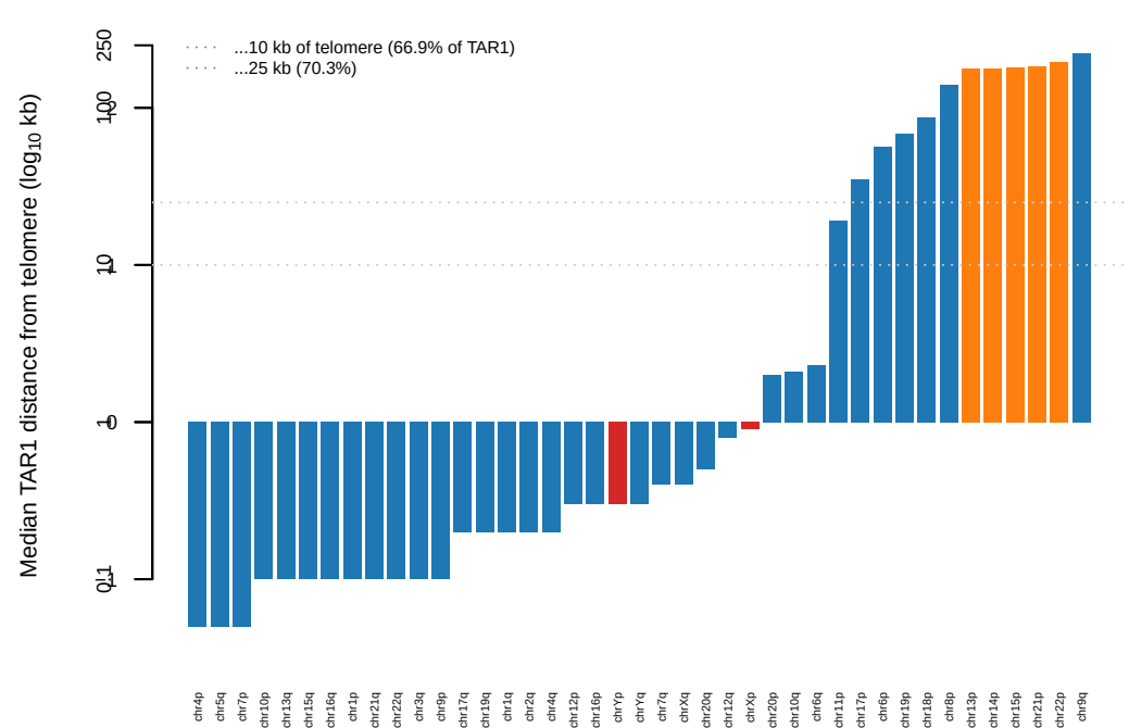
d Per-arm TAR1 distance-from-telomere
