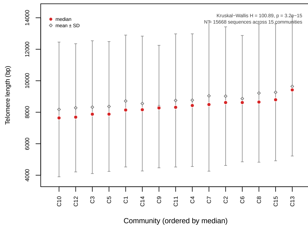
c Terminal telomere length by community
