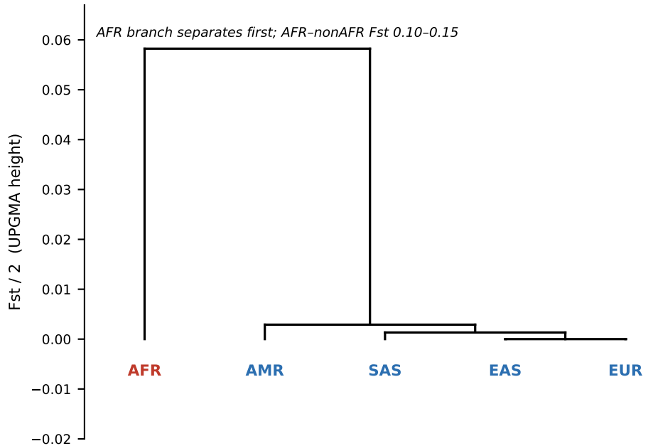
d Out-of-Africa tree from cross-arm F_{st}
