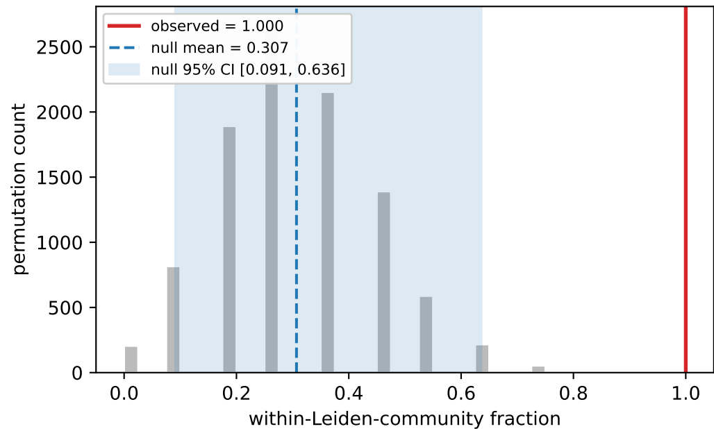
CEPH1463 cross-assembler (n=11)
