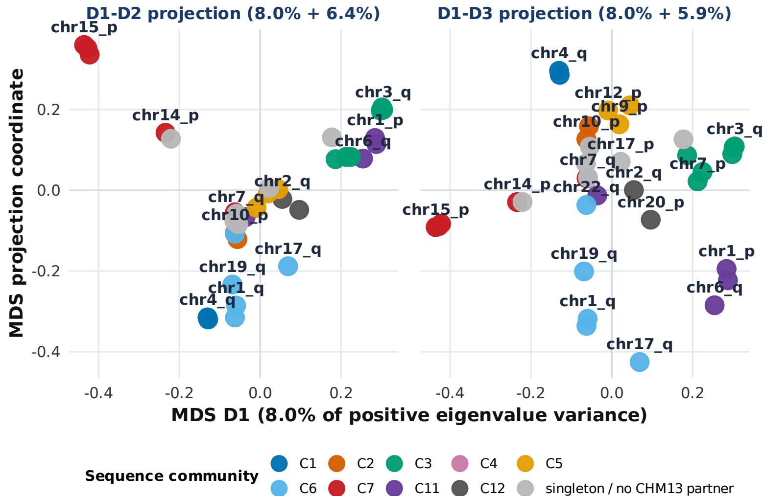
Caption: CHM13 Hi-C contact-space MDS over PHR/subtelomeric arm regions from chm13_subtelomeric_regions.bed at 50 kb resolution, shown as D1-D2 and D1-D3 projections of a 3D MDS. Colors mark sequence-defined subtelomeric communities; nearby points indicate similar bulk Hi-C contact profiles. This is contact-space MDS from bulk Hi-C, not a physical single-cell genome reconstruction.
