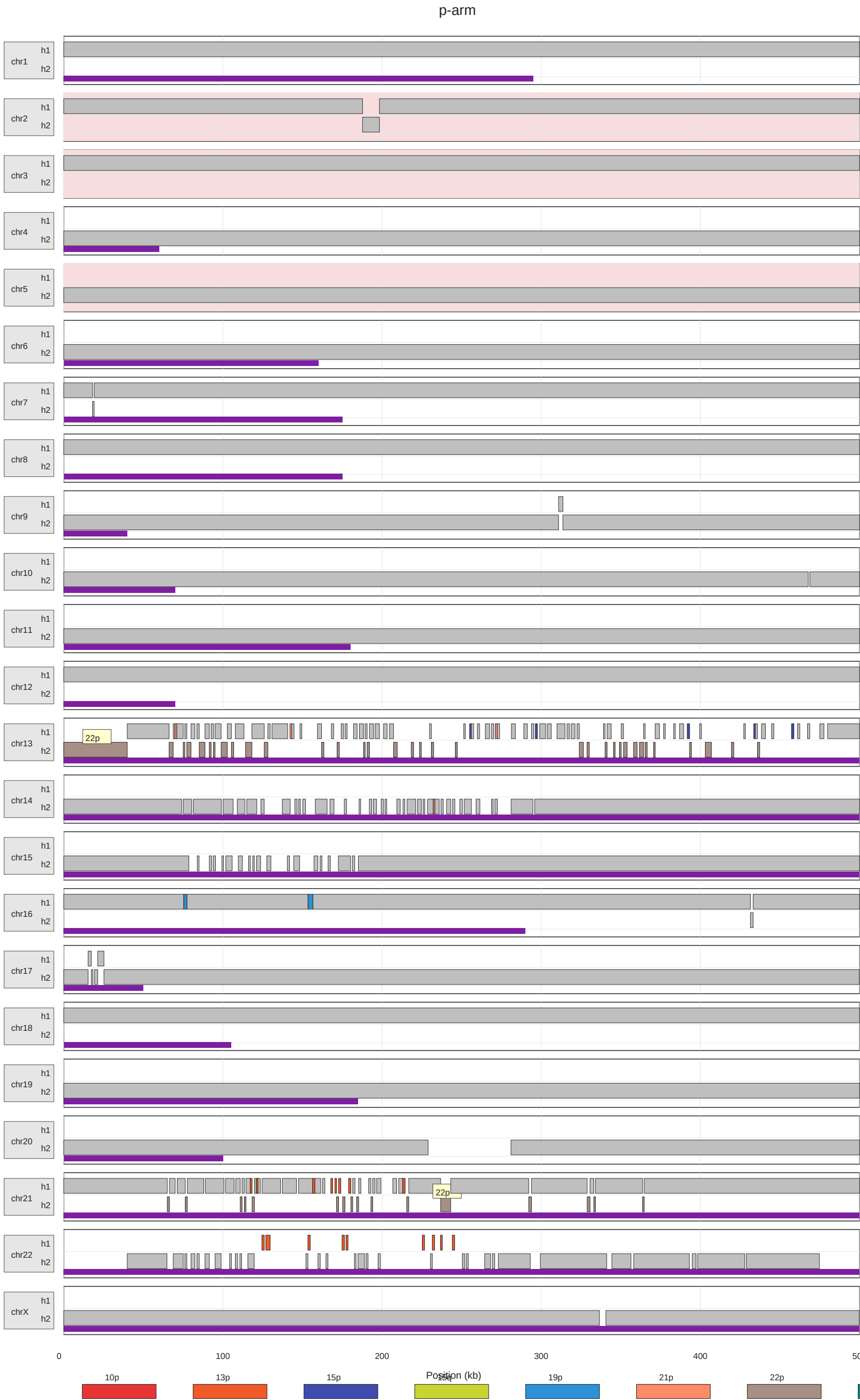
PAN027 maternal hap1 <- PAN010 mother - conservative sweepGA 1:1, submitted-style view
