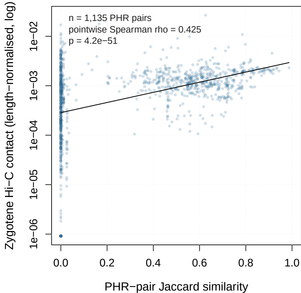
Mouse: sequence-similar PHR pairs contact more
