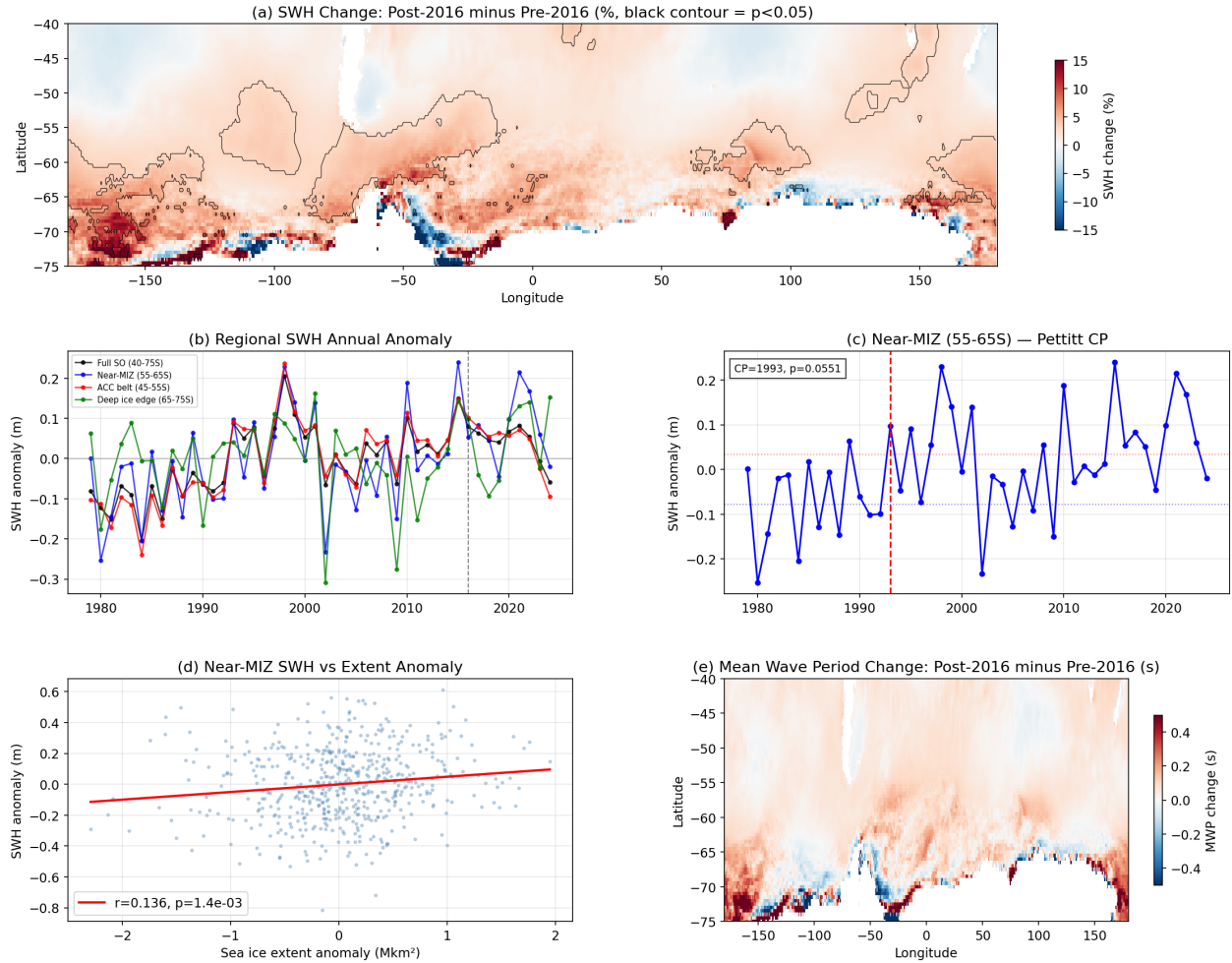
Figure 2: ERA5 significant wave height trends in the Southern Ocean (1979–2024). a , Spatial map of SWH percentage change (post-2016 minus pre-2016). Black contours enclose regions where the change is significant ( p < 0.05 , two-sample t -test). Widespread increases are concentrated in the ACC belt. b , Regional annual SWH anomaly time series for four latitude bands. c , Near-MIZ zone (55–65°S) Pettitt change point at 1993 ( p = 0.055 ). d , SWH anomaly versus sea ice extent anomaly ( r = 0.136 ). e , Mean wave period change (post-2016 minus pre-2016).
