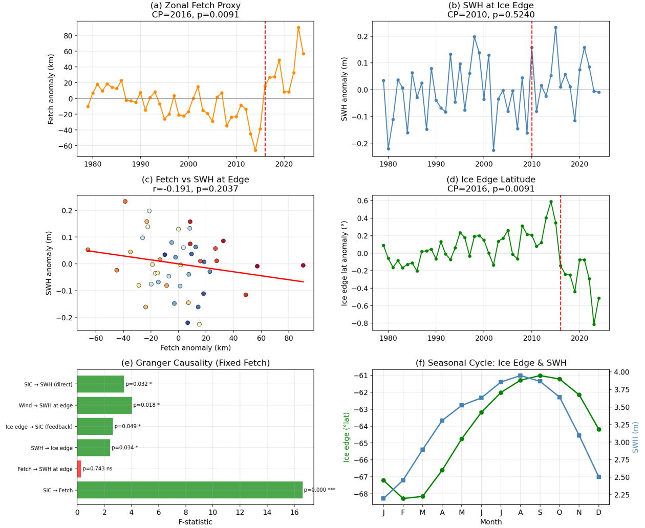
Figure 3: Ice-edge-based fetch proxy and SWH at the ice edge (1979–2024). a , Zonal-mean fetch proxy (distance from 40°S to ice edge) annual anomaly. Change point at 2016 ( p = 0.009 ). b , SWH sampled at the ice edge. No significant change point ( p = 0.52 ). c , Scatter plot of fetch anomaly versus SWH at the ice edge ( r = -0.19 , p = 0.20 ): fetch does not predict SWH. d , Ice-edge latitude anomaly with change point at 2016. e , Granger causality F -statistics. Green = significant ( p < 0.05 ); orange = marginal; red = not significant. f , Seasonal cycle of fetch and SWH at the ice edge.
