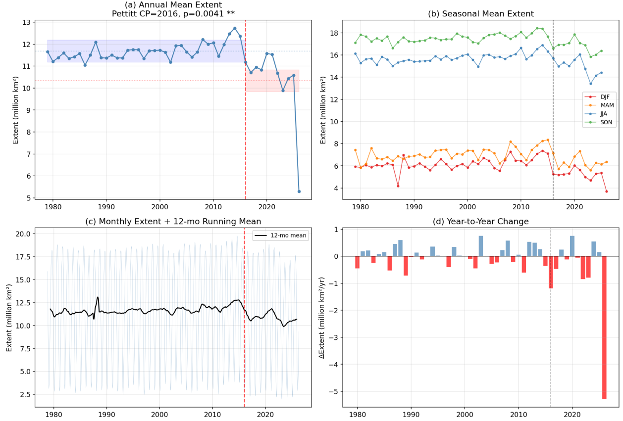
Figure 1: Antarctic sea ice extent baseline (NSIDC Sea Ice Index, 1979–2026). a , Annual mean extent with Pettitt change point at 2016 ( p = 0.004 ). Blue/red shading indicates pre/post-shift mean levels. b , Seasonal mean extent (DJF, MAM, JJA, SON). Summer (DJF) shows the largest post-2016 decline ( -16.8\% ). c , Monthly extent with 12-month running mean. d , Year-to-year change, showing the abrupt shift to persistent negative anomalies after 2016.
