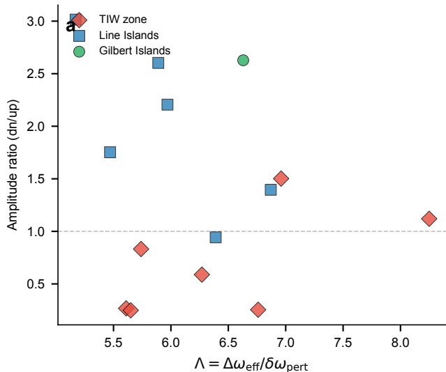
(a) Real GLORYS-derived \Lambda vs robustness
