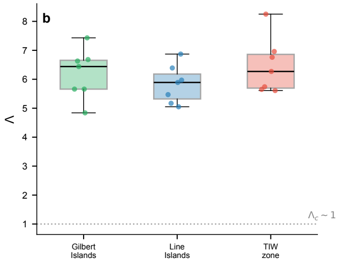
(b) \Lambda distribution by perturbation zone
