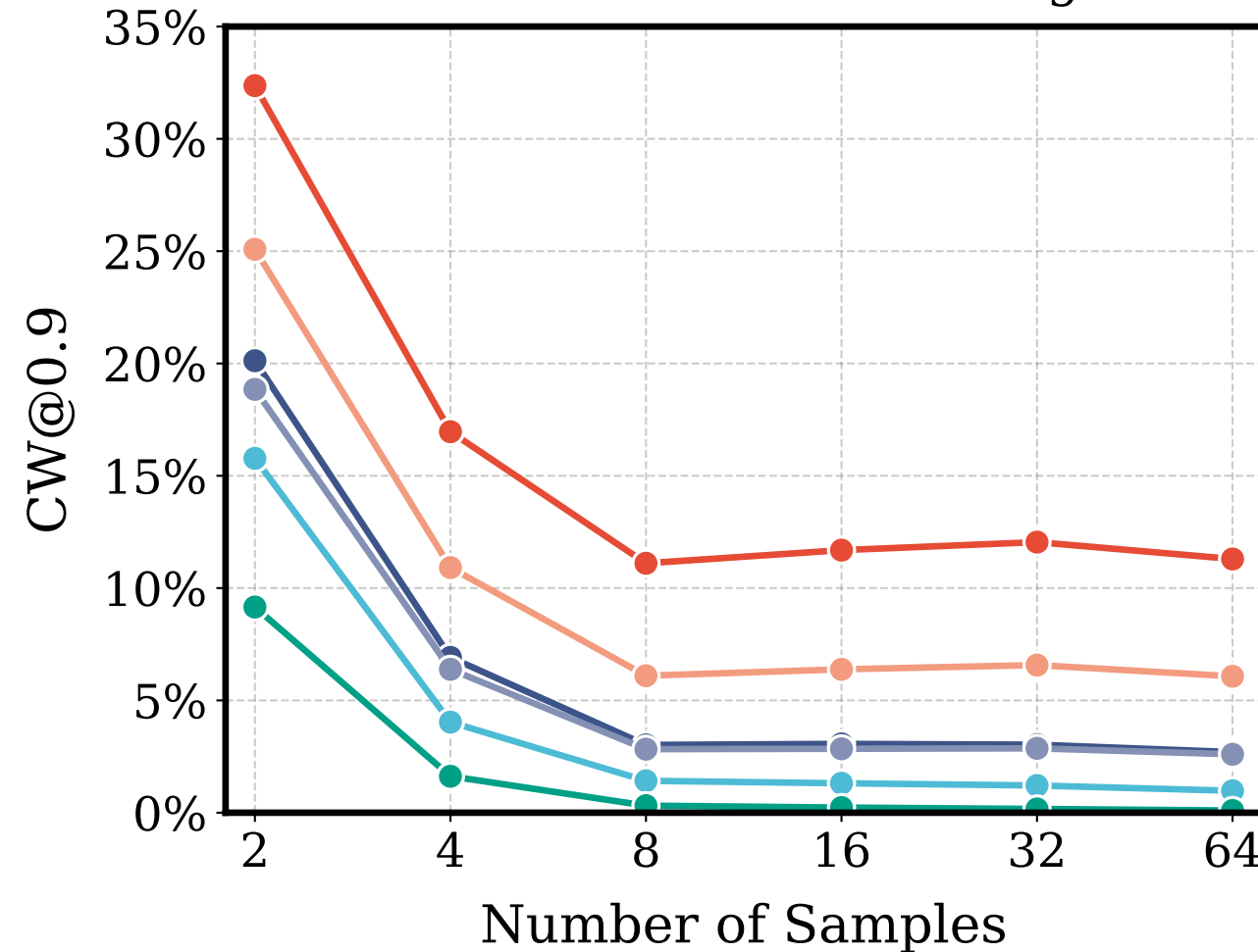
(b) More samples do not eliminate confident wrongs
