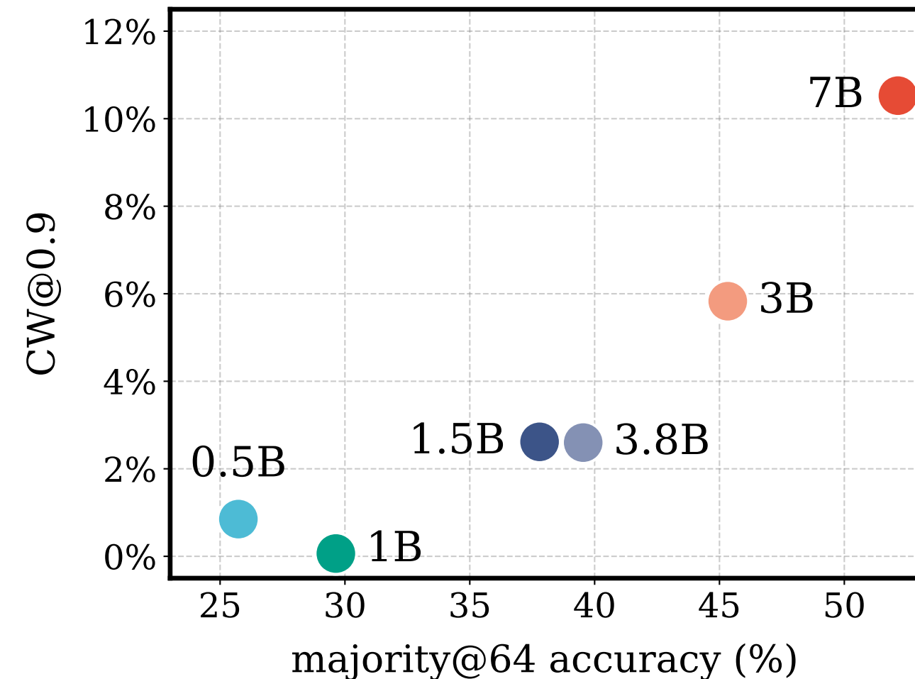
(c) Stronger models are more confidently wrong
