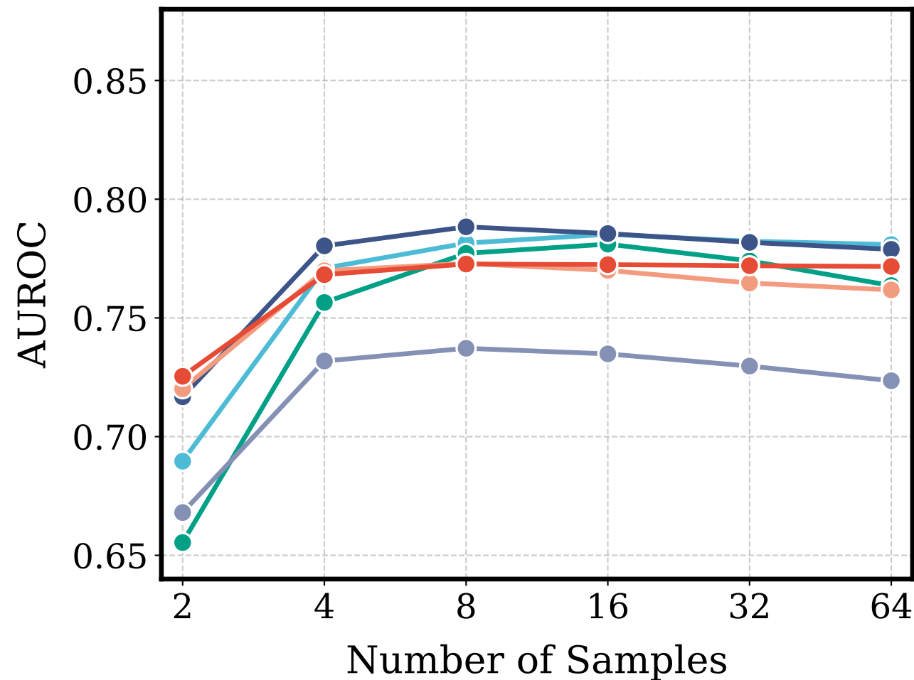
(a) Answer-level UQ saturates with sampling
