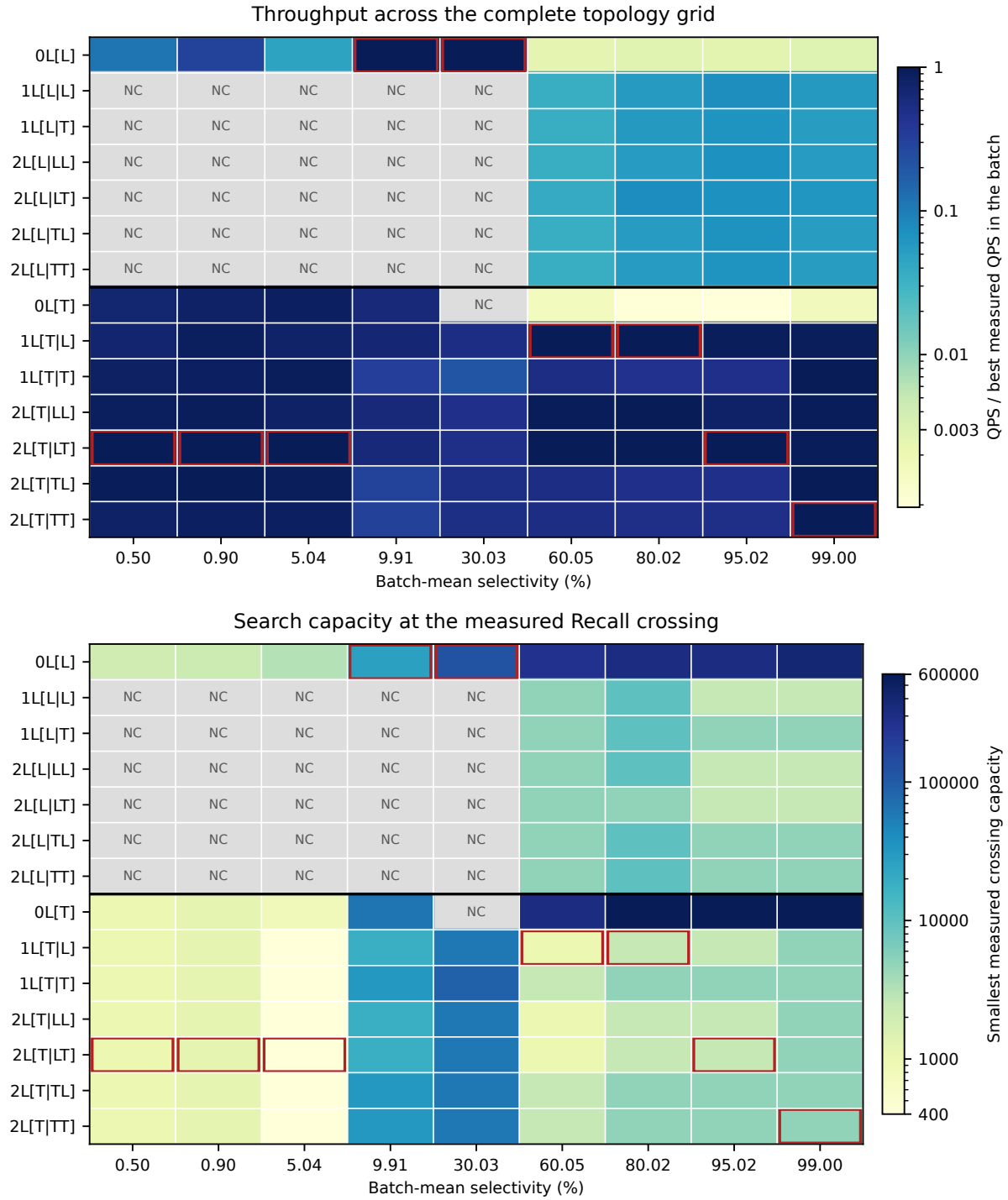
Figure 5: Complete 14-configuration grid: QPS relative to the largest measured QPS in each batch (top), and the selected search capacity (bottom). Both use the same Recall crossings, logarithmic color scales, and fixed thresholds. A red border marks the measured QPS winner in both panels. Grey NC cells have no crossing within the common measured budget. Cross-base comparisons use matched entry providers.
