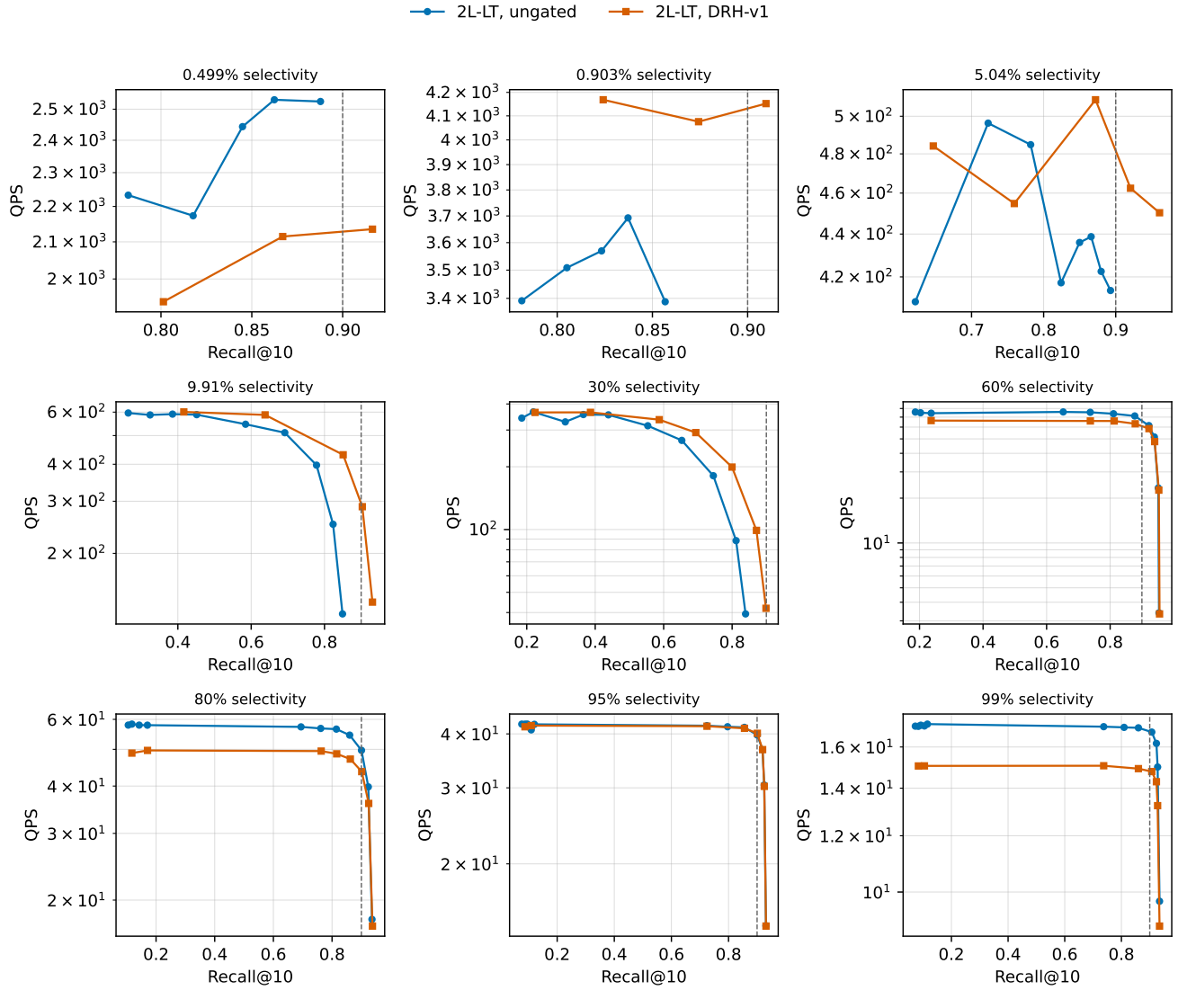
Figure 9: Measured Recall@10-QPS curves for ungated versus DRH-v1 routing for 2L[L|LT]. Markers are executed points; curves are not interpolated.
