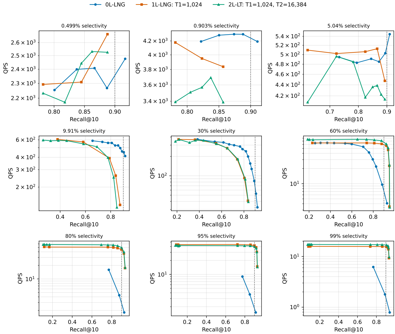
Figure 8: Measured Recall@10-QPS curves for the representative 0L/1L/2L comparison. Markers are executed points; curves are not interpolated.
