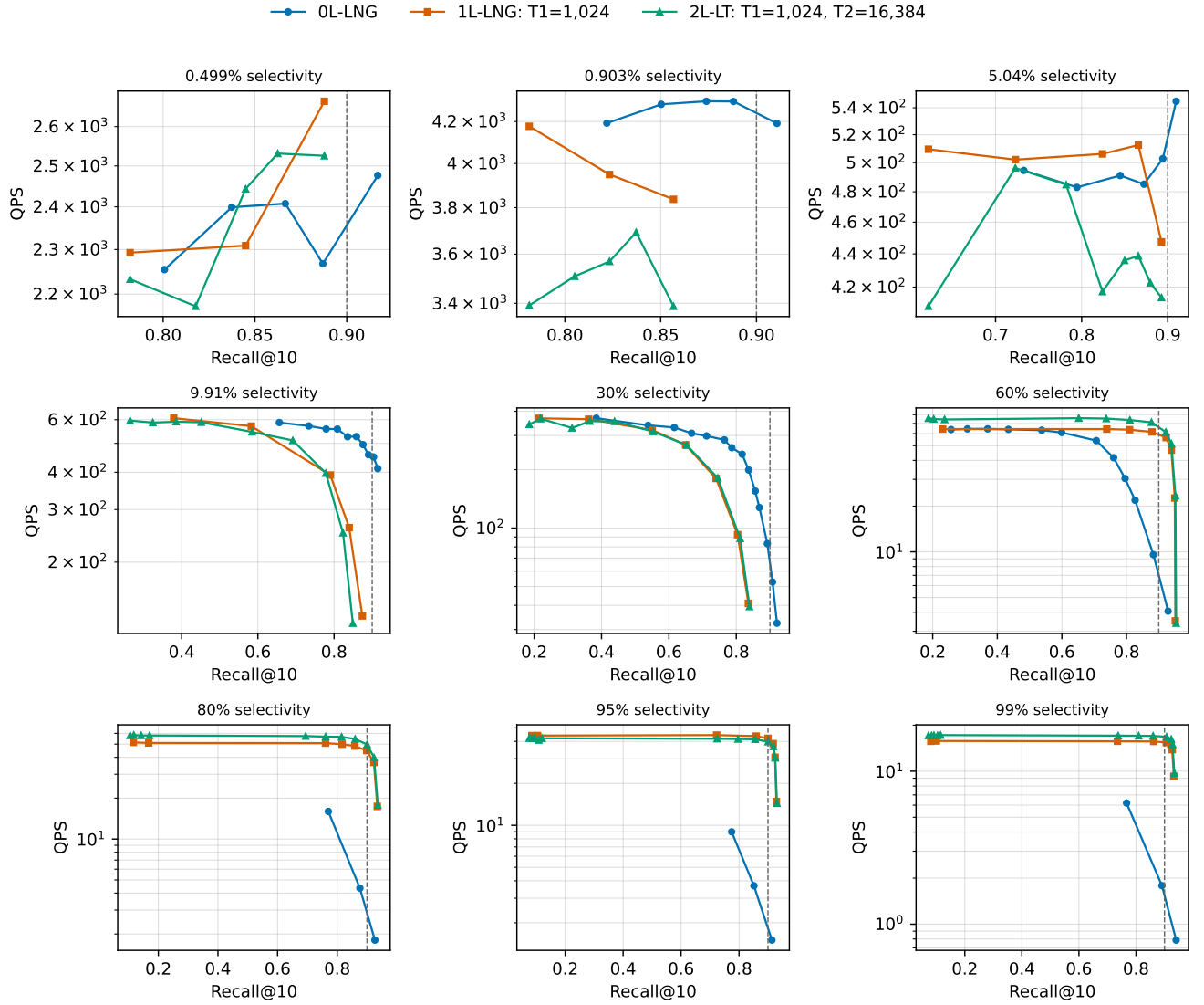
Figure 9: Measured Recall@10-QPS curves for the representative 0L/1L/2L comparison. Markers are executed points; curves are not interpolated.
