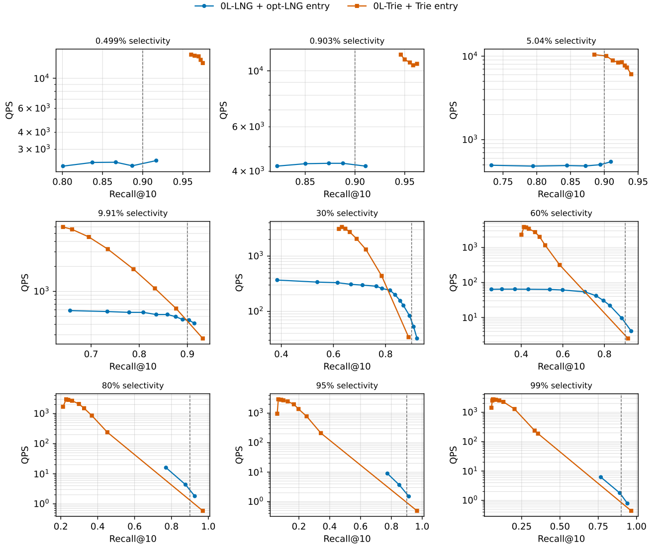
Figure 7: Measured Recall@10-QPS curves for the 0L[L]/0L[T] comparison. Markers are executed points; curves are not interpolated.
