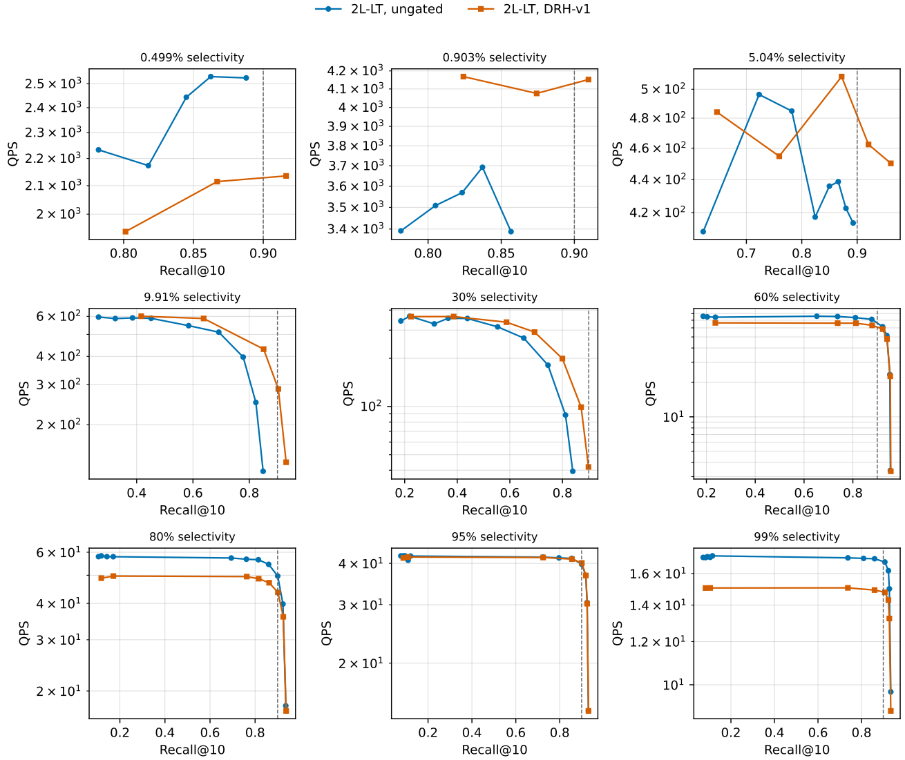
Figure 10: Measured Recall@10-QPS curves for ungated versus DRH-v1 routing for 2L[L|LT]. Markers are executed points; curves are not interpolated.
