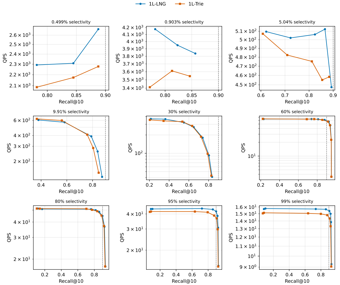
Figure 8: Measured Recall@10-QPS curves for 1L[L]/1L[T] overlay topology at fixed threshold, level-0 LNG, and entry provider. Markers are executed points; curves are not interpolated.
