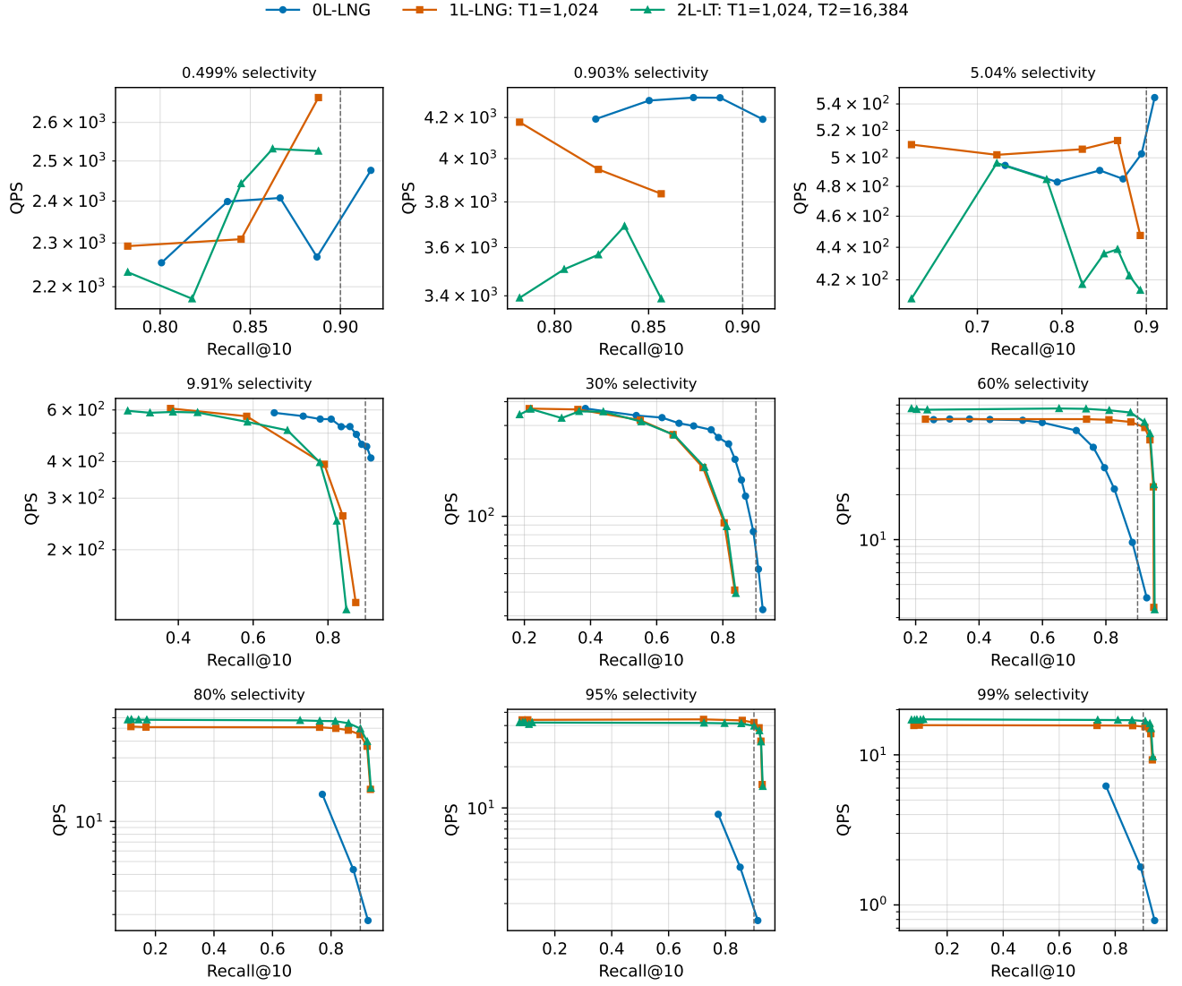
Figure 4: Measured Recall@10-QPS curves for the representative 0L/1L/2L comparison. Markers are executed points; curves are not interpolated.
