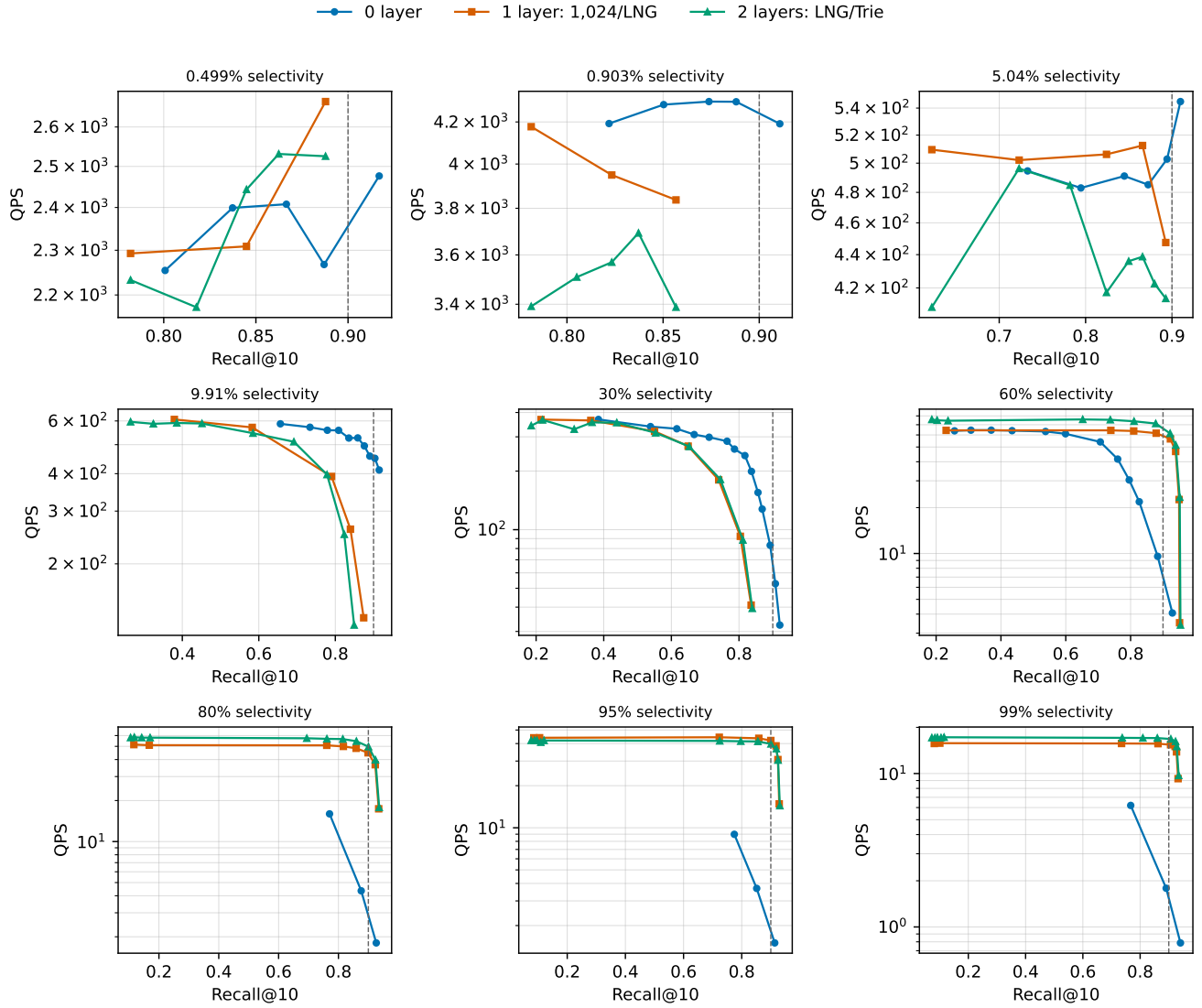
Figure 3: Measured Recall@10-QPS curves for the representative zero/one/two-layer comparison. Markers are executed points; curves are not interpolated.
