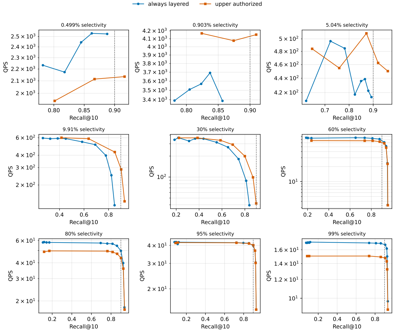
Figure 4: Measured Recall@10-QPS curves for the upper-layer authorization ablation. Markers are executed points; curves are not interpolated.
