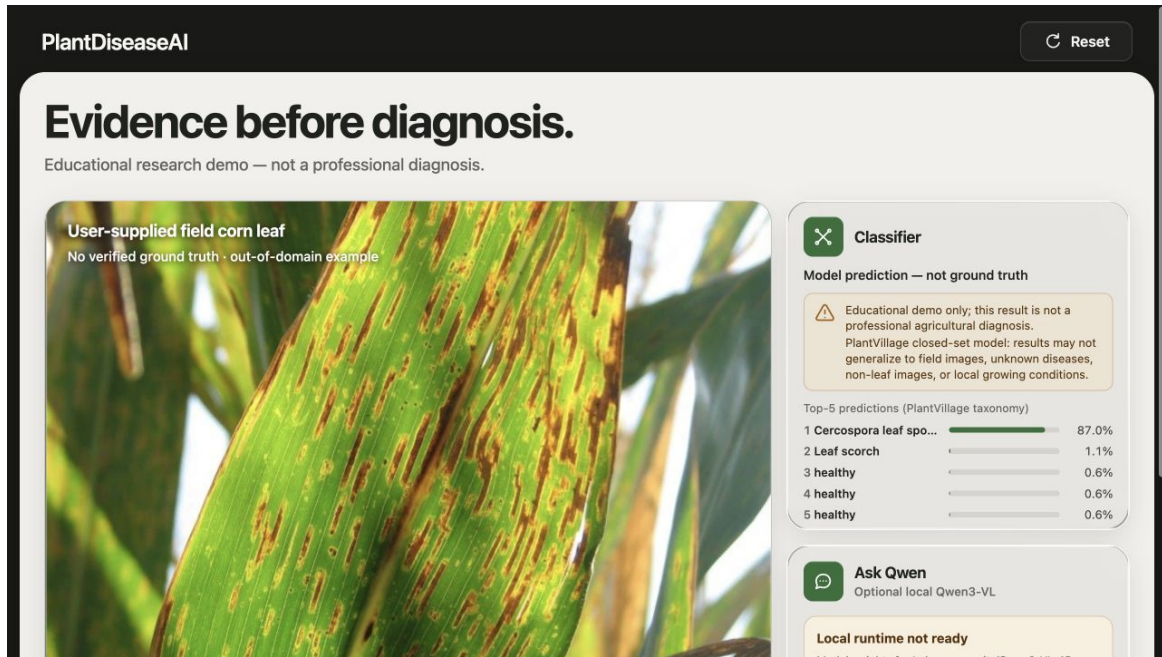
Figure 4: Browser-audited Week 8 React Demo. The ResNet-50/MPS value 0.870144 is a prediction, not truth or field-accuracy evidence; the image has no verified label and lies outside the controlled PlantVillage domain.
