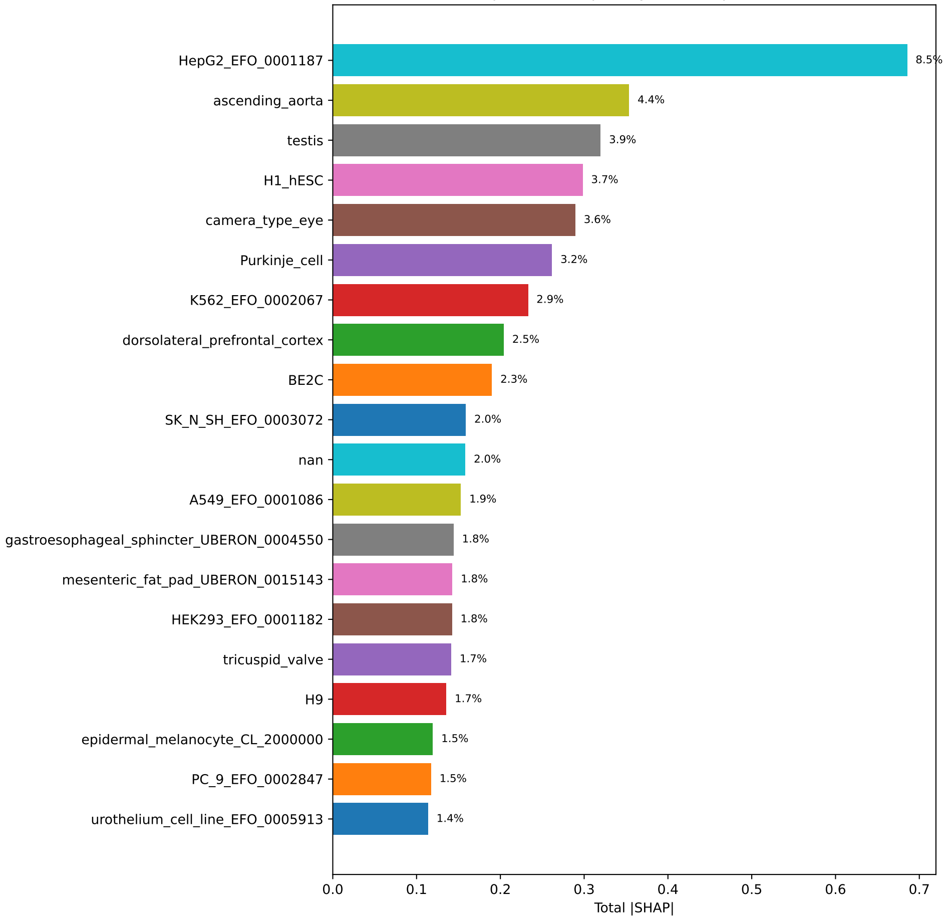
Top 20 biosamples by SHAP importance
