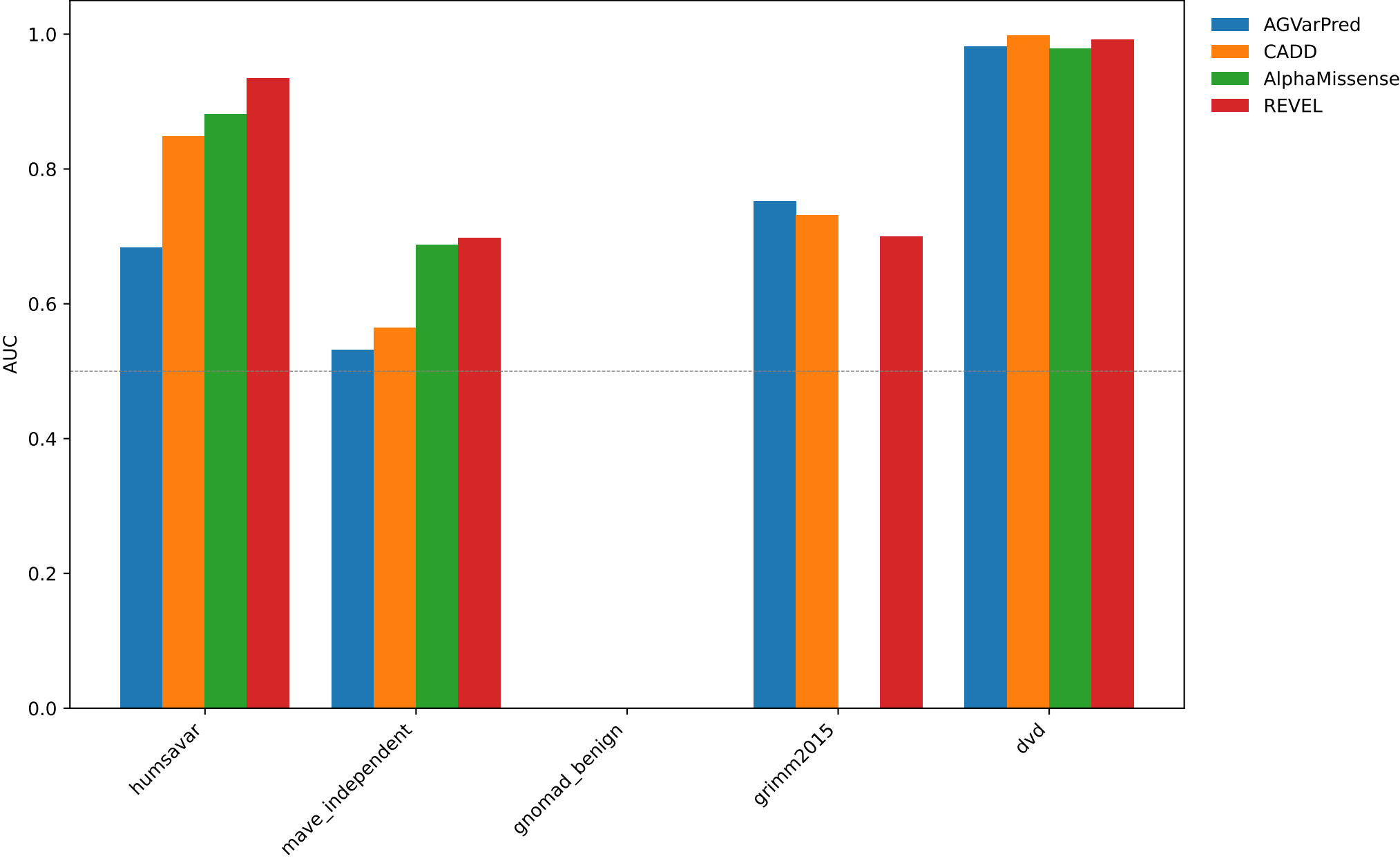
Non-missense variant performance
