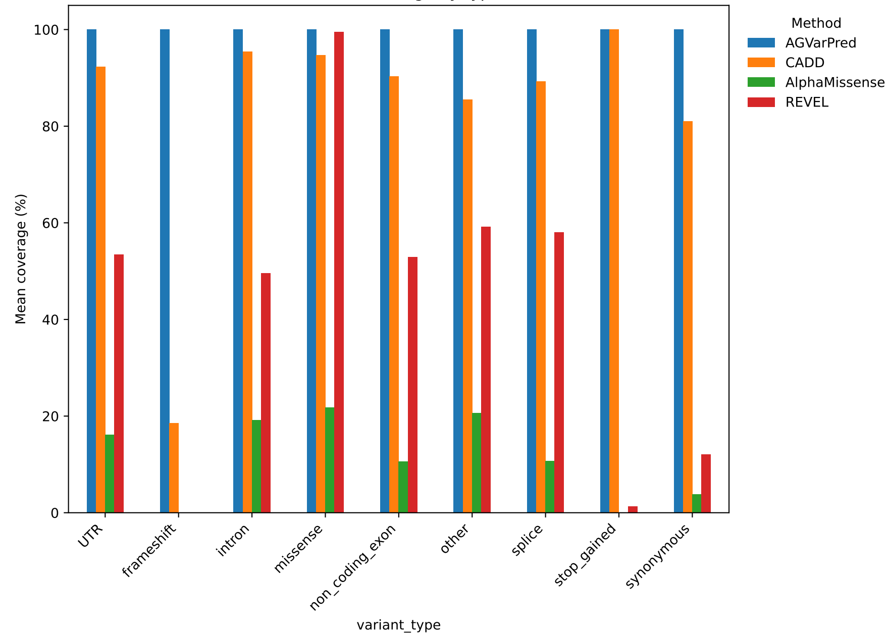
Variant coverage by type
