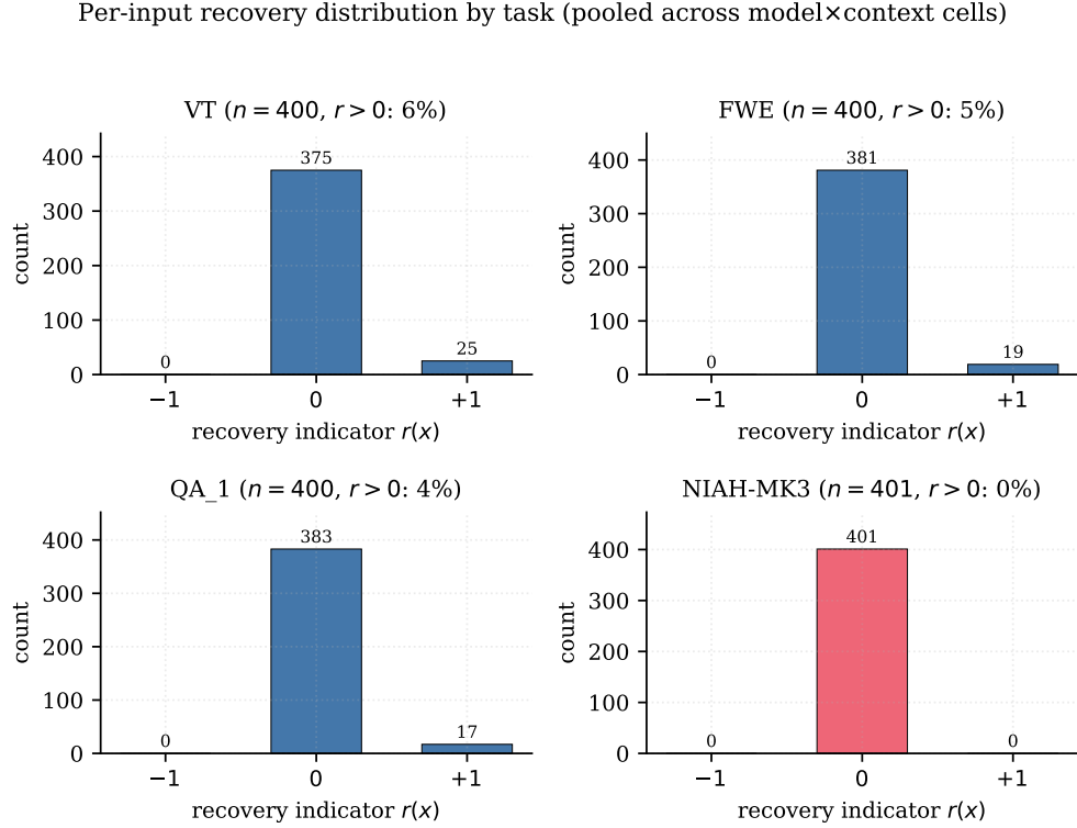
Figure 8: Per-input recovery indicator r(x) pooled across model and context cells, faceted by RULER task. The three dilution-prone tasks show a non-trivial right tail at r=+1 with zero mass at r=-1 ; NIAH-MK3 is concentrated entirely at r=0 , consistent with the capacity-bound regime.
