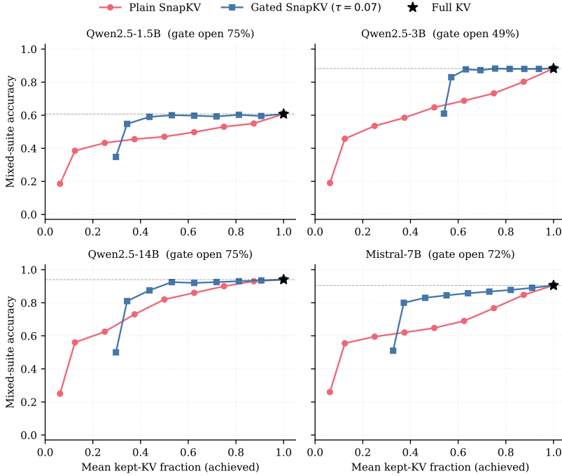
Figure 3: Accuracy vs. achieved kept-KV fraction (mean over inputs of n_{\text{kept}}/T ) on the mixed 4K suite (NIAH-MK3 + VT + FWE + QA_1), SnapKV. Because the gate falls back to the full cache when it closes, gated points sit at larger kept-KV than their nominal budget; the honest comparison is at matched achieved cache size. For every target kept-KV fraction \gtrsim 1/3 (Qwen3B: \gtrsim 0.57 ) the gated curve is the Pareto frontier, by up to +19pp over plain at equal cache size; at the most aggressive nominal budget ( b = 0.0625 , leftmost gated point) the gated point is dominated by plain eviction at a matched cache size, and \tau = 0.07 caps achievable compression at 1 - \text{open-fraction} of the cache (0.25–0.51 across models). All gated results use the post-hoc \tau = 0.07 reconstruction (Appendix H); the reconstruction reproduces the stored gated outcomes exactly on the three runs executed at \tau = 0.07 .
