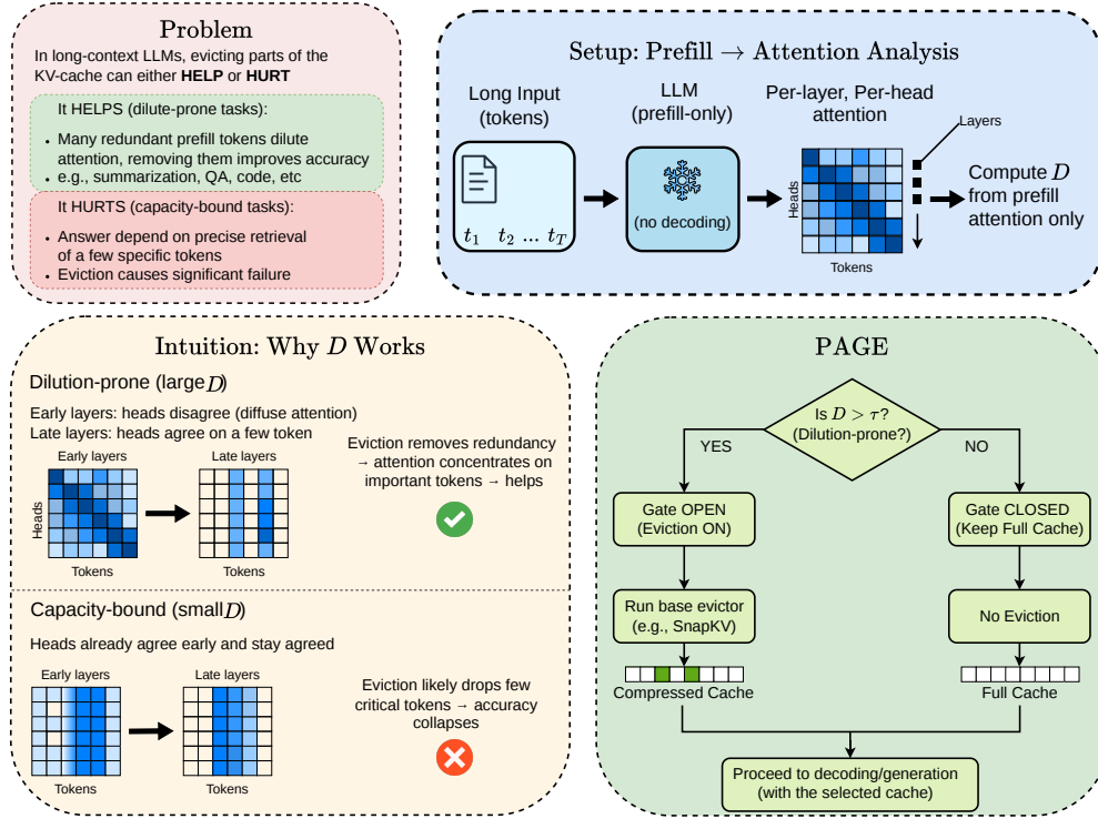
Figure 1: The head-agreement drop D separates the two task classes. The gate closes below the line (keep the full cache) and opens above it (run the base evictor).
