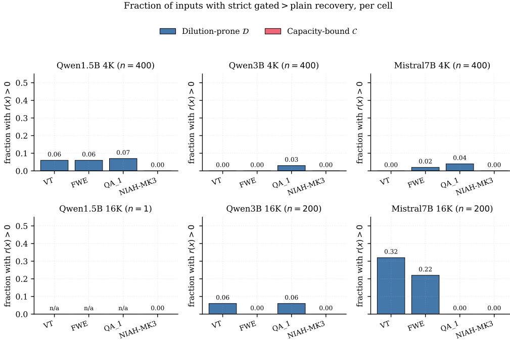
Figure 9: Fraction of inputs with strict recovery r(x) > 0 per task, faceted by (model, context) cell. Dilution-prone bars are non-trivial in every cell with data, while NIAH-MK3 stays at or near zero, visualising the partition input by input.
