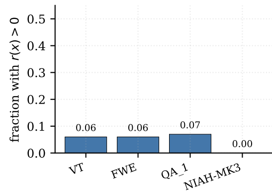
Qwen1.5B 16K ( n = 1 )
