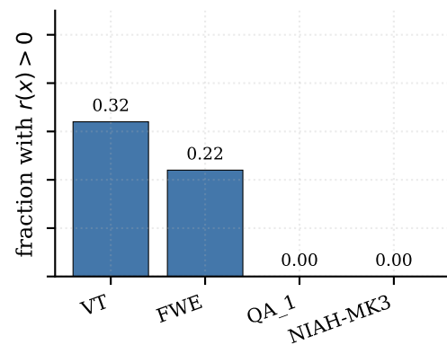
Mistral7B 16K ( n = 200 )
