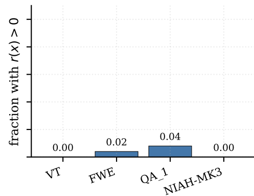
Mistral7B 16K ( n = 200 )
