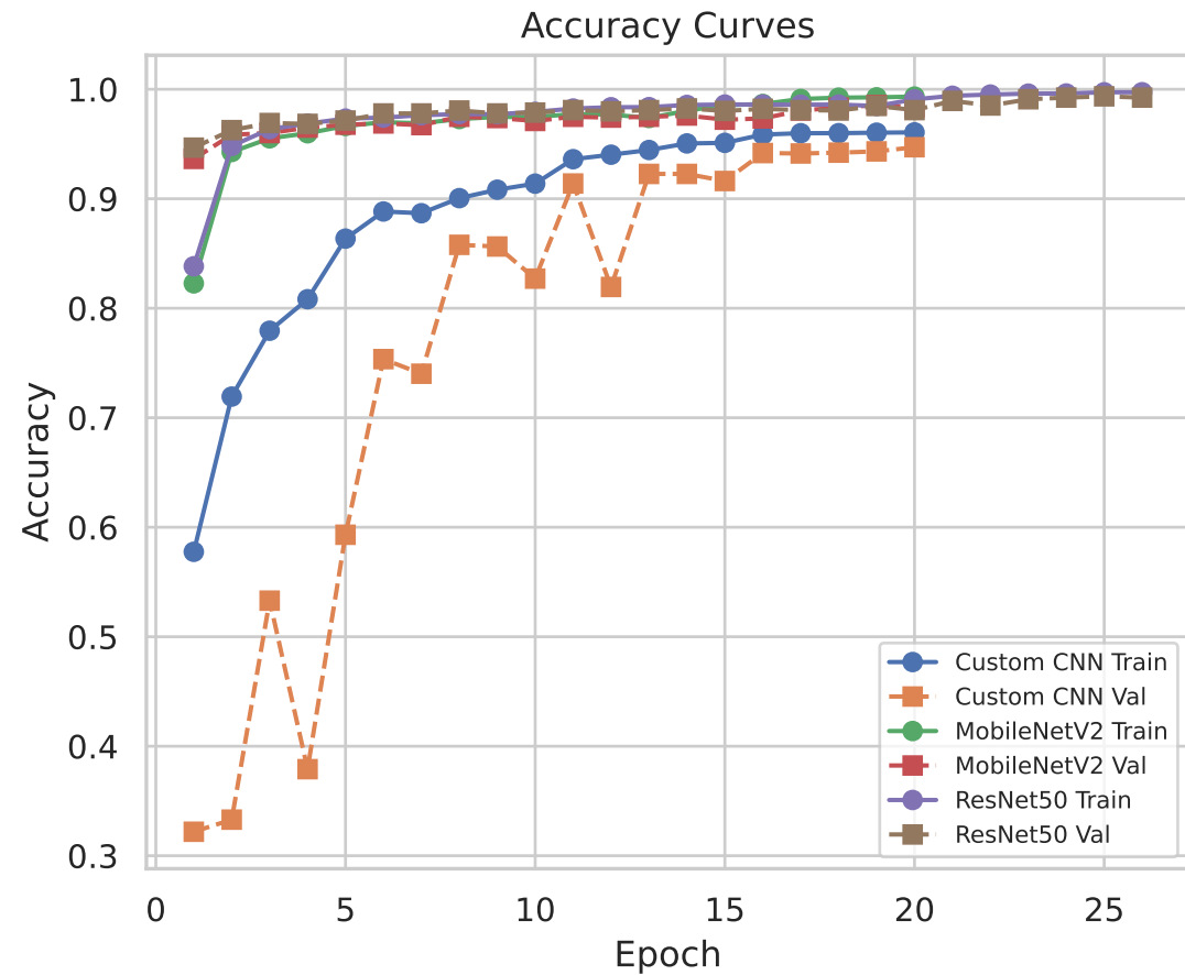
Figure 3: Accuracy and Loss Curves
