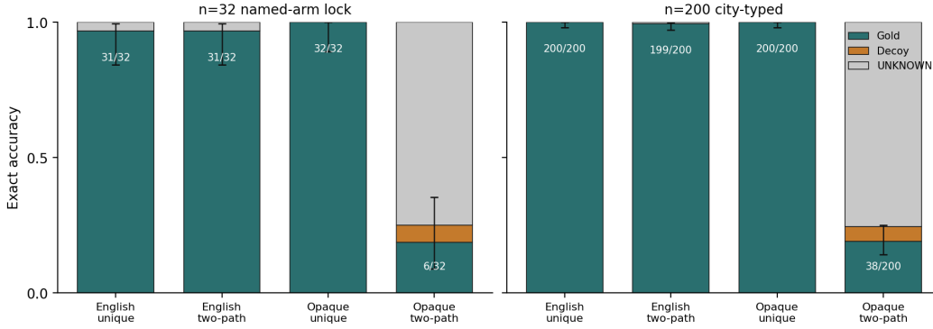
Figure 1: OpenAI WIKI-H5 2 \times 2 (start in q ). Stacked bars are gold / decoy / UNKNOWN; whiskers are Wilson 95% intervals. Left: n=32 named-arm lock (August; opaque two-path 6/32). Right: city-typed n=200 freeze (named-arm opaque two-path 38/200, UNKNOWN 151, decoy 11). Hashed-id 134/200 and alias k=3 are Section 5.2.
