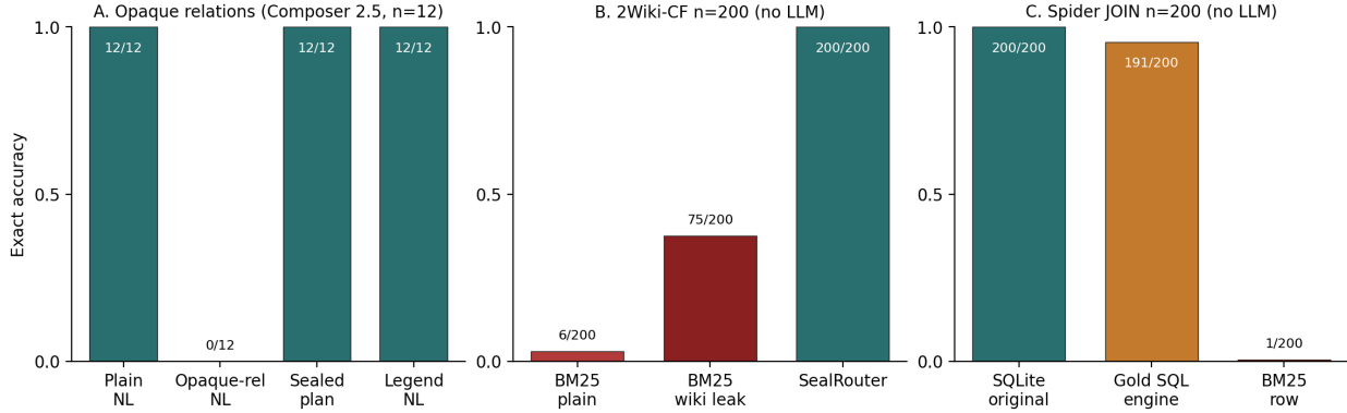
Figure 3: Non-LLM and packaging controls. Left: Composer n=12 (plain 12/12, opaque-rel NL 0/12, plan 12/12). Middle: 2Wiki-CF BM25 6/200, Wikipedia leak 75/200, SealRouter 200/200. Right: Spider sqlite 200/200, gold-SQL 191/200, BM25 1/200.
