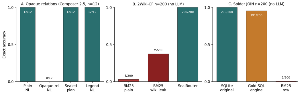
Figure 5: Non-LLM and packaging controls. Left: opaque-rel restore (Composer 2.5, n=12 ). Middle: 2Wiki-CF BM25 6/200 vs. SealRouter 200/200. Right: Spider engine vs. BM25. CEO/2Wiki opacity \times prompt-form scores are in the surrounding prose.
