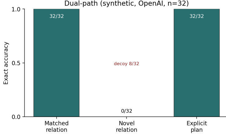
Figure 2: DUAL (synthetic, OpenAI n=32 ): matched 32/32; novel 0/32 (asymmetric decoy 8).
