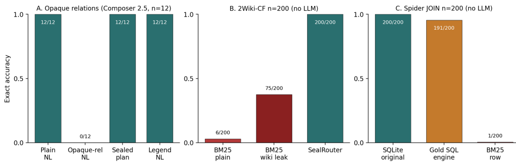
Figure 5: Non-LLM and packaging controls (file fig7_opaque_rel_n200.png). Panel A is Composer n=12 ; panels B–C are frozen n=200 baselines. Left: opaque-rel NL 0/12 vs. plan/legend 12/12 (Composer 2.5, n=12 ). Middle: 2Wiki-CF BM25 6/200, Wikipedia-string leak 75/200, SealRouter 200/200. Right: Spider sqlite 200/200, gold-SQL engine 191/200, BM25 1/200. CEO/2Wiki opacity \times prompt-form scores are in the surrounding prose.
