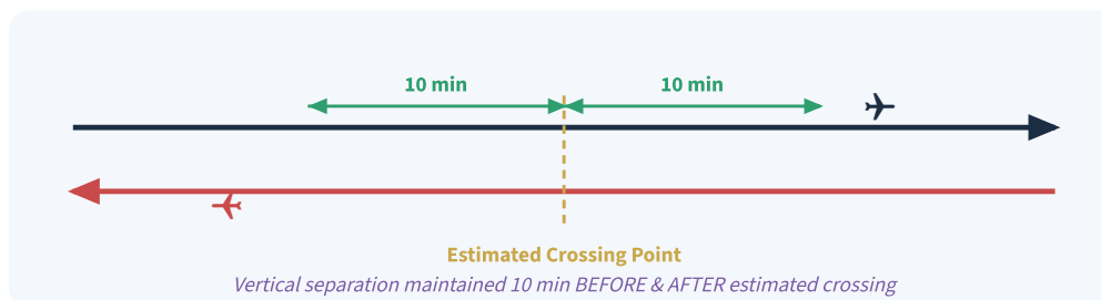
Fig 4.1 — 10-Minute Separation on Reciprocal Tracks
