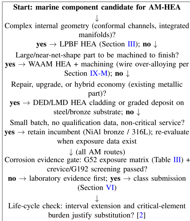
Fig. 3. Decision tree for route selection and deployment gating of AM-HEA marine components, linked to the indicative cost model (Table VI). All decision logic is proposal [P]; the cost anchors behind it are flagged in Section IX-N.
