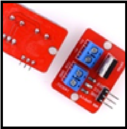
0-24V IFR520 MOS Driver Module Board SKU:-HW-042
