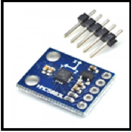
Digital Compass Module - HMC5883L I2C Output
