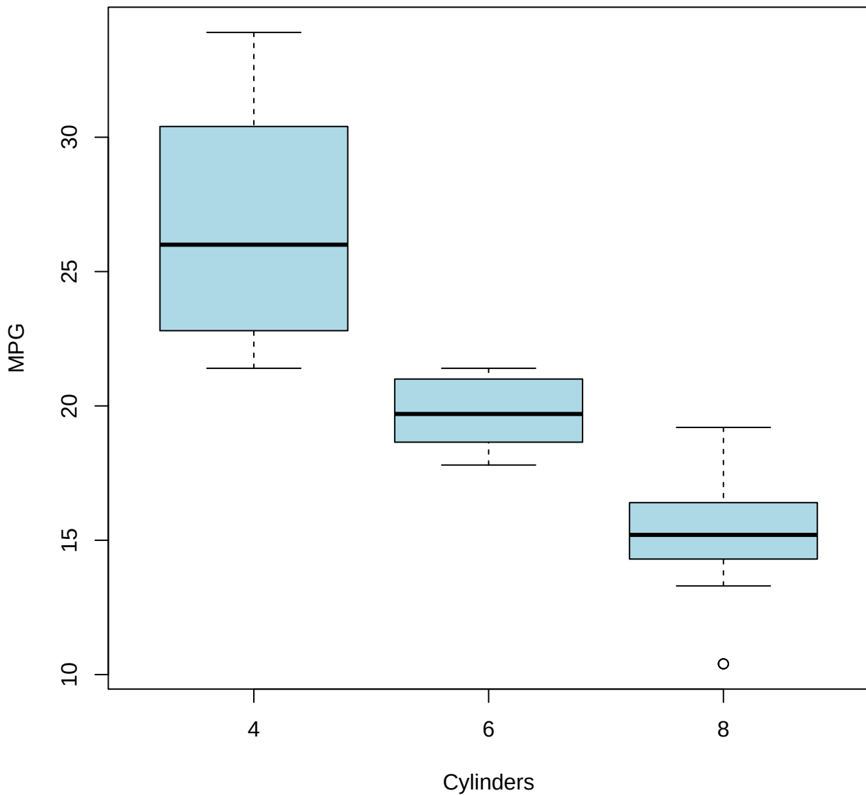
MPG by Cylinder Count
