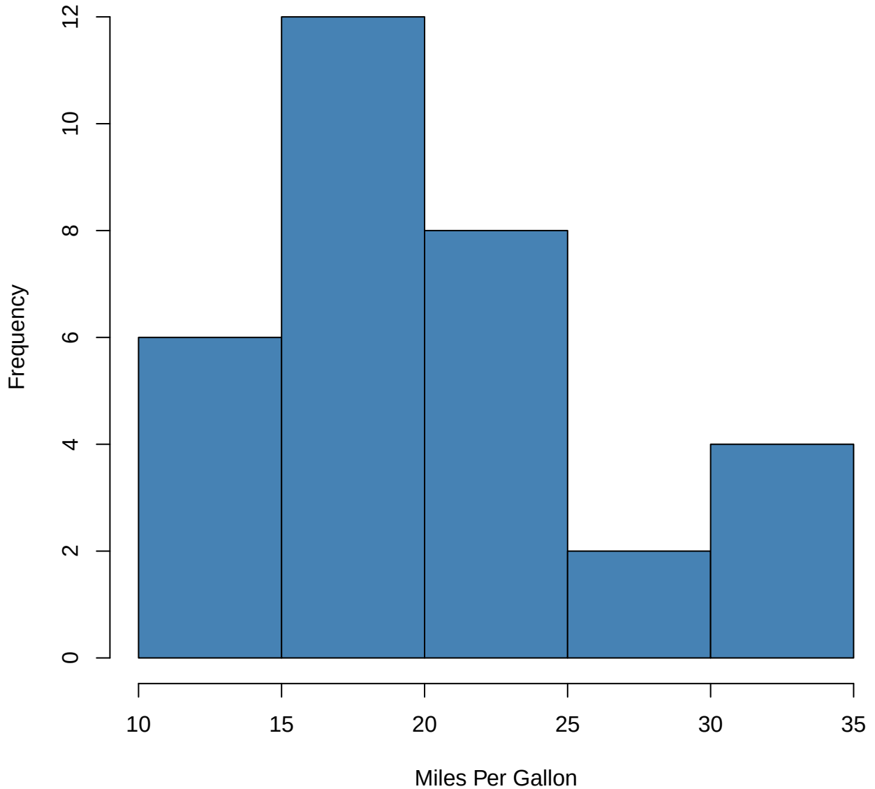
Histogram of MPG
