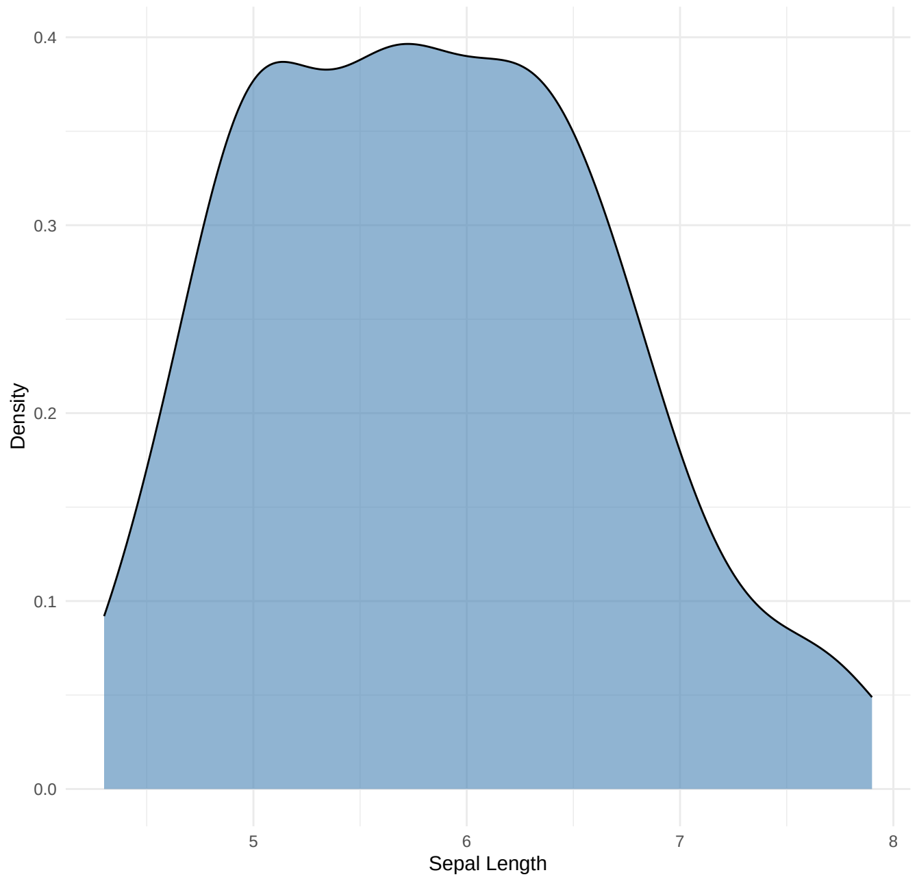
Density of Sepal.Length
