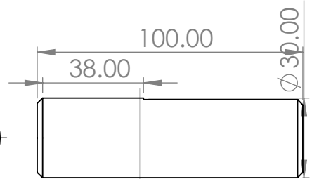
PIN
