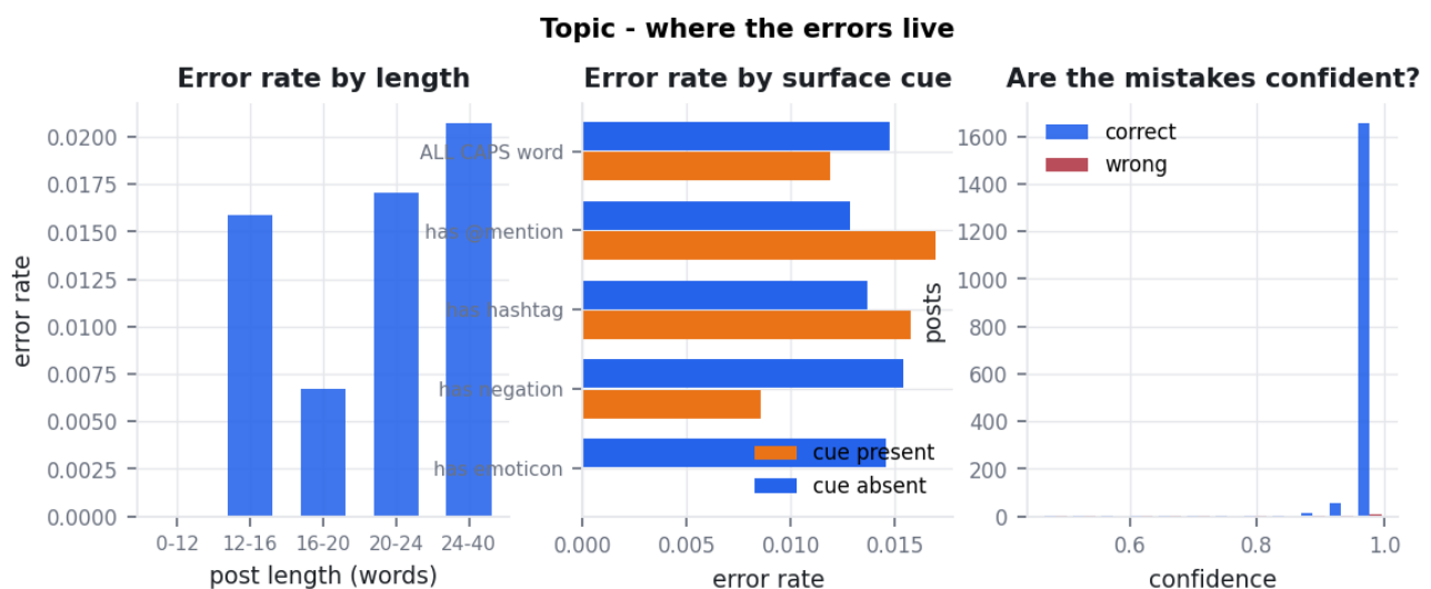
Figure 12. Topic errors by length, surface cue and confidence.
