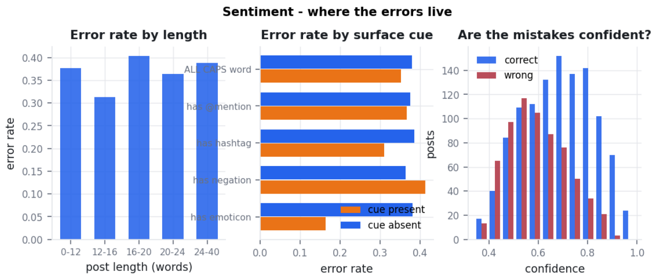
Figure 11. Sentiment errors by length, surface cue and confidence.
